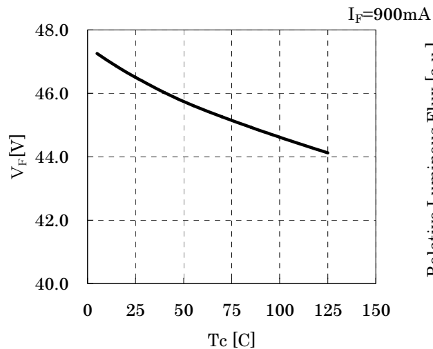
• Case Temperature vs. Forward Voltage
