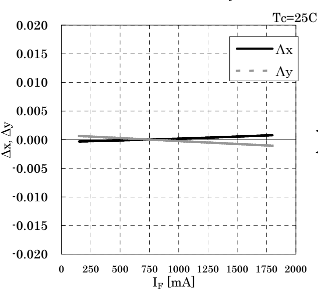
•Forward Current vs. Chromaticity Coordinate
