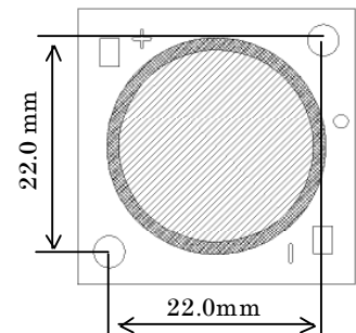
Recommended installation screw pitch
