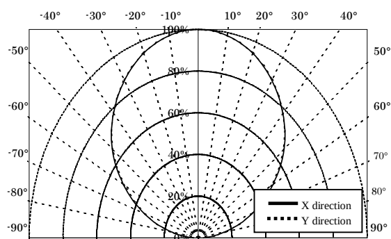
•Directive Characteristic
