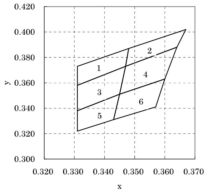
x-y chart-CIE 1931
