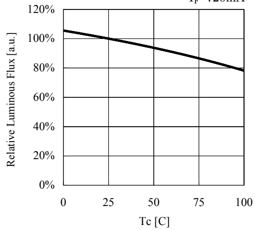
Case Temperature vs. Relative Luminous Flux I_F=720\text{mA}
