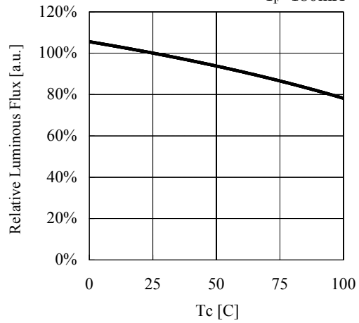
Case Temperature vs. Relative Luminous Flux I_F=180\text{mA}
