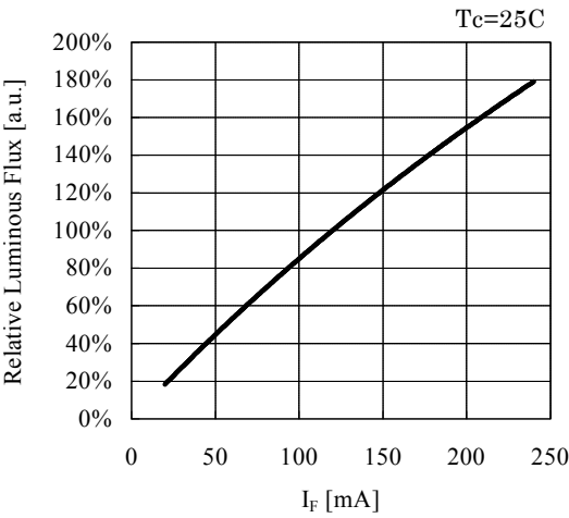
Forward Current vs. Relative Luminous Flux
