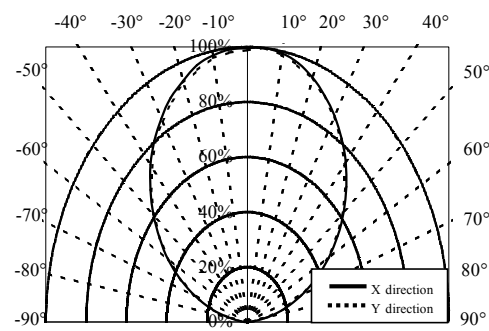
Directive Characteristic
