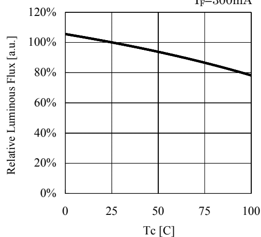
•Case Temperature vs. Relative Luminous Flux I_F=300\text{mA}
