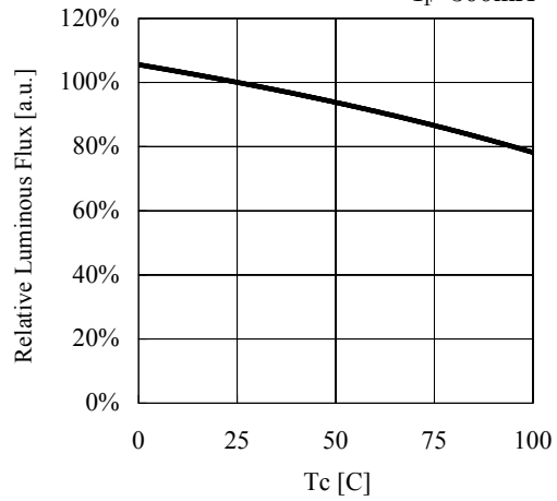
Case Temperature vs. Relative Luminous Flux I_F=300\text{mA}
