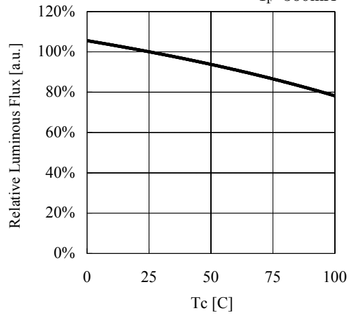
Case Temperature vs. Relative Luminous Flux I_F=360\text{mA}
