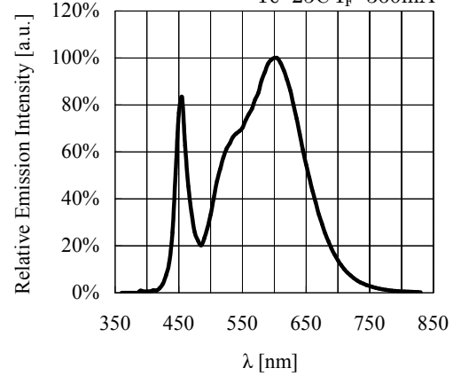
Spectrum T_c=25^\circ\text{C} I_F=360\text{mA}
