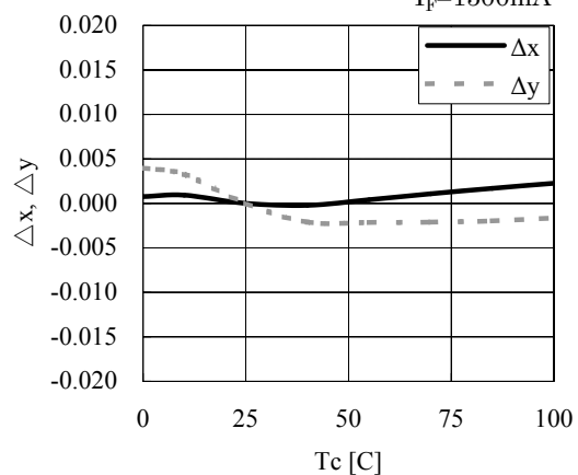
Case Temperature vs. Chromaticity Coordinate
