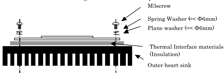
Recommended installation screw pitch
