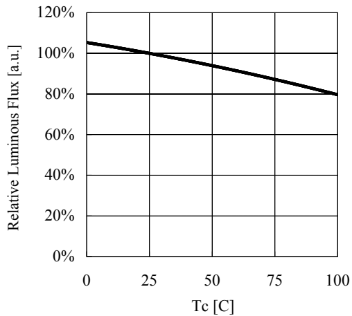
Case Temperature vs. Relative Luminous Flux IF=360mA
