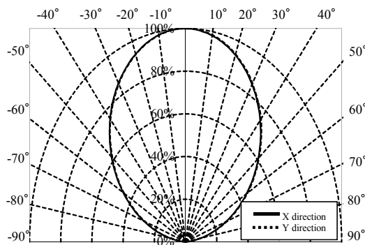
Directive Characteristic
