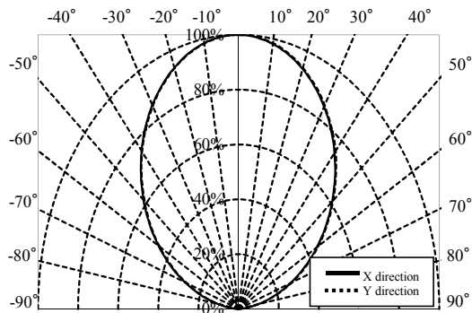
Directive Characteristic
