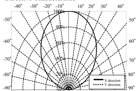
Directive Characteristic
