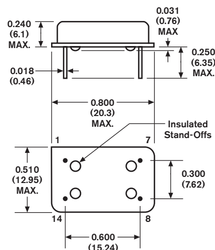
FULL SIZE 14 PIN DIP
