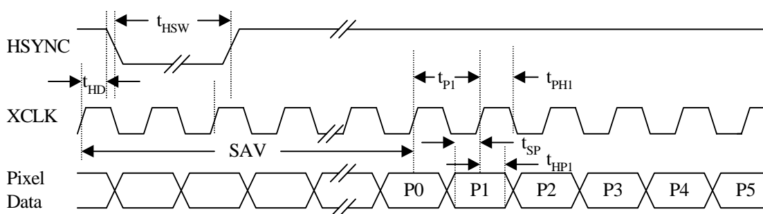
Figure 4: Non-multiplexed Data Transfers
