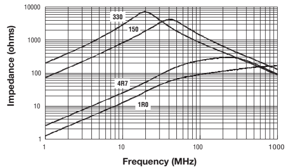
Impedance Characteristics
