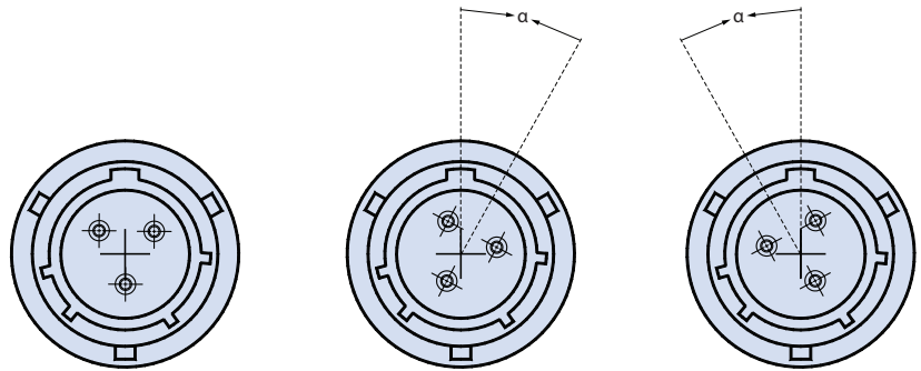
Normal Position Alternate Position with Pin Contacts Alternate Position with Socket Contacts
