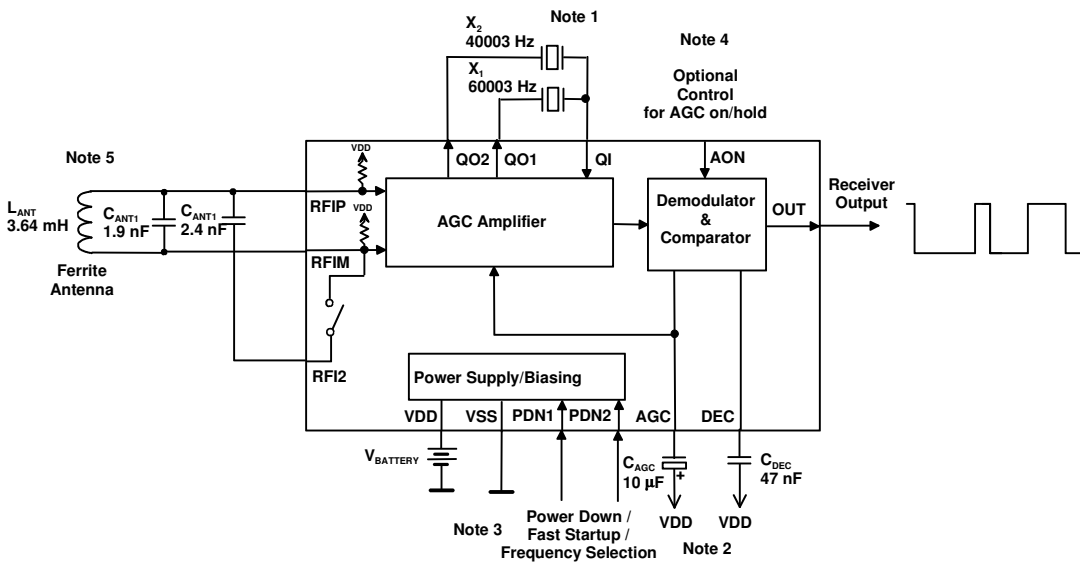
Figure 2. Example circuit of dual band receiver MAS6181 for JYJ 60 kHz and 40 kHz frequencies
