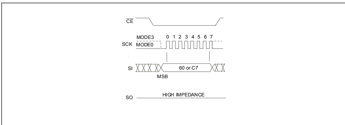
Figure 16: Chip Erase Sequence
