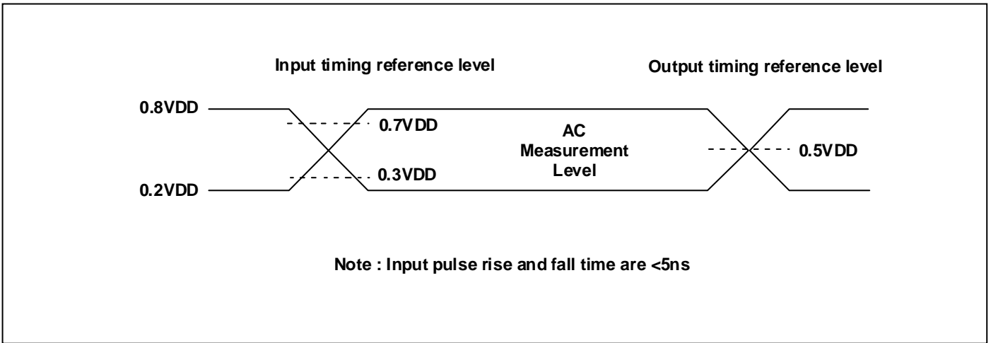
Figure 34: AC Input/Output Reference Waveforms
