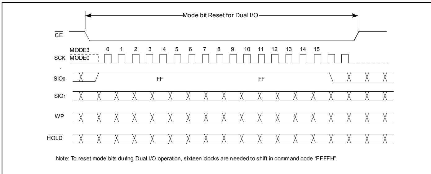
Figure 8: Mode Bit Reset Instruction
