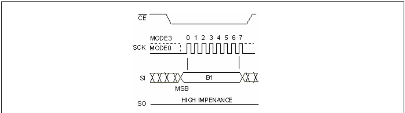
Figure 19: Enter OTP Mode (ENSO) Sequence
