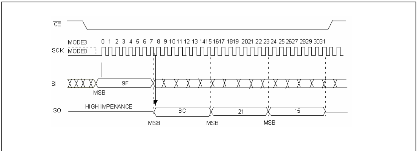
Figure 23: JEDEC Read-ID Sequence
