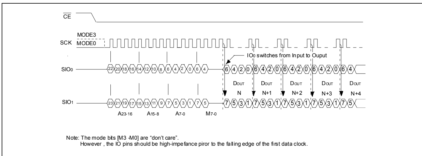
Figure 6: Fast Read Dual I/O Sequence ( [M_7-M_0] = \text{AxH} )
