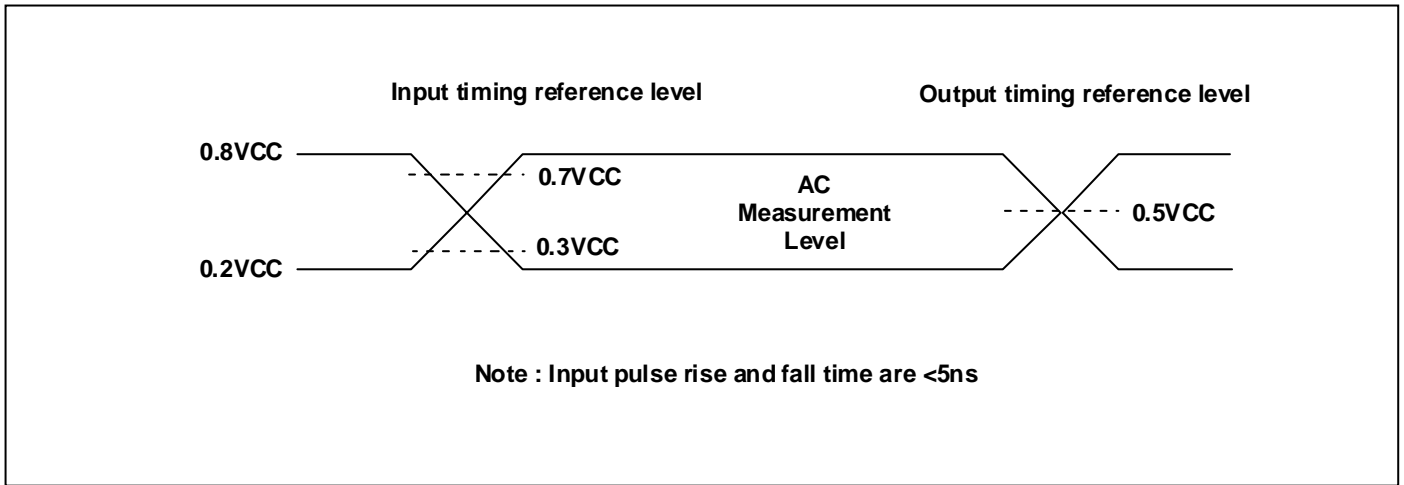
Figure 30: AC Input/Output Reference Waveforms
