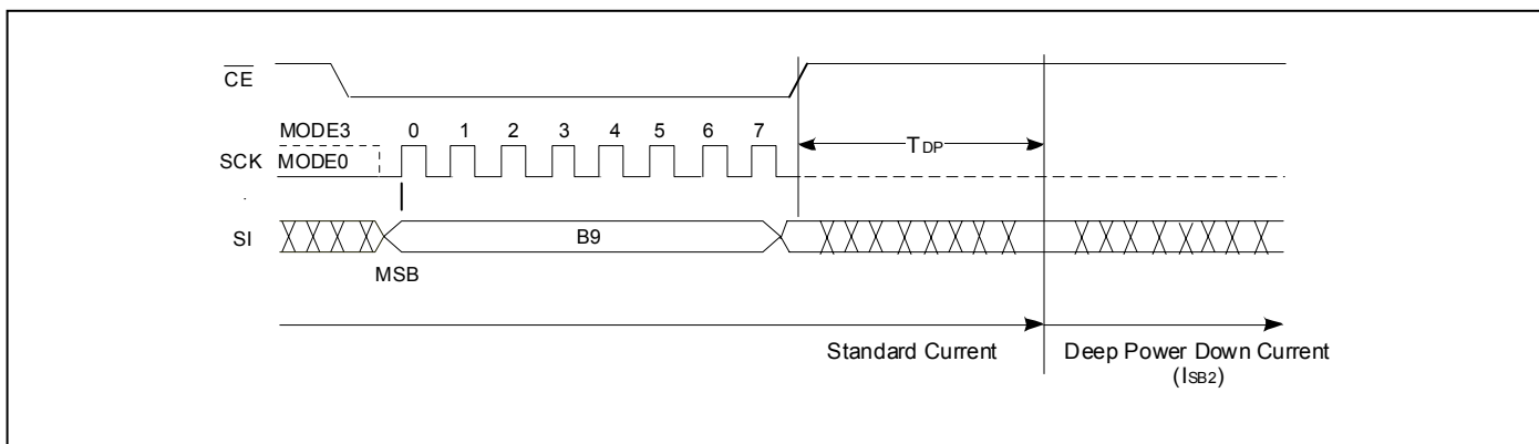
Figure 20: Deep Power Down Instruction
