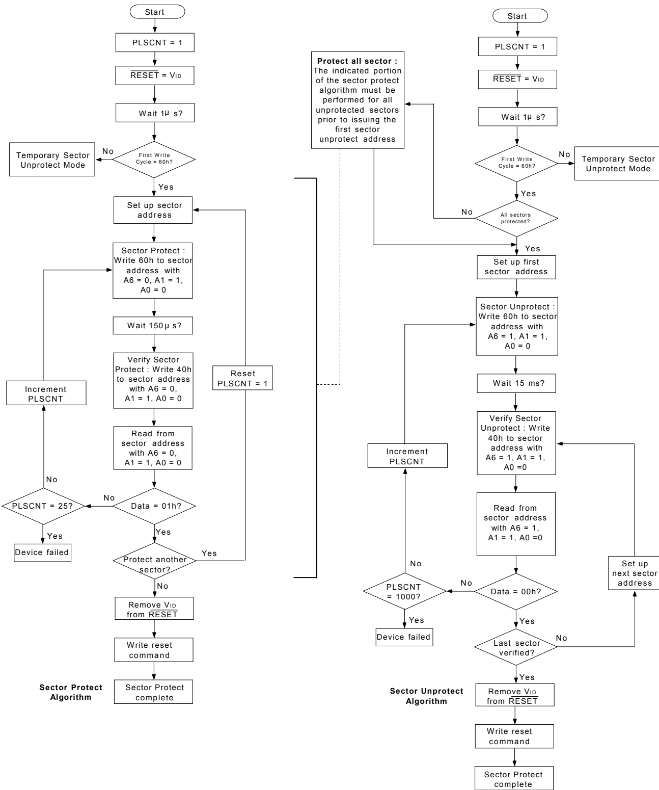
Figure 16. In-System Sector Protect/Unprotect Algorithm (RESET = V ID )
