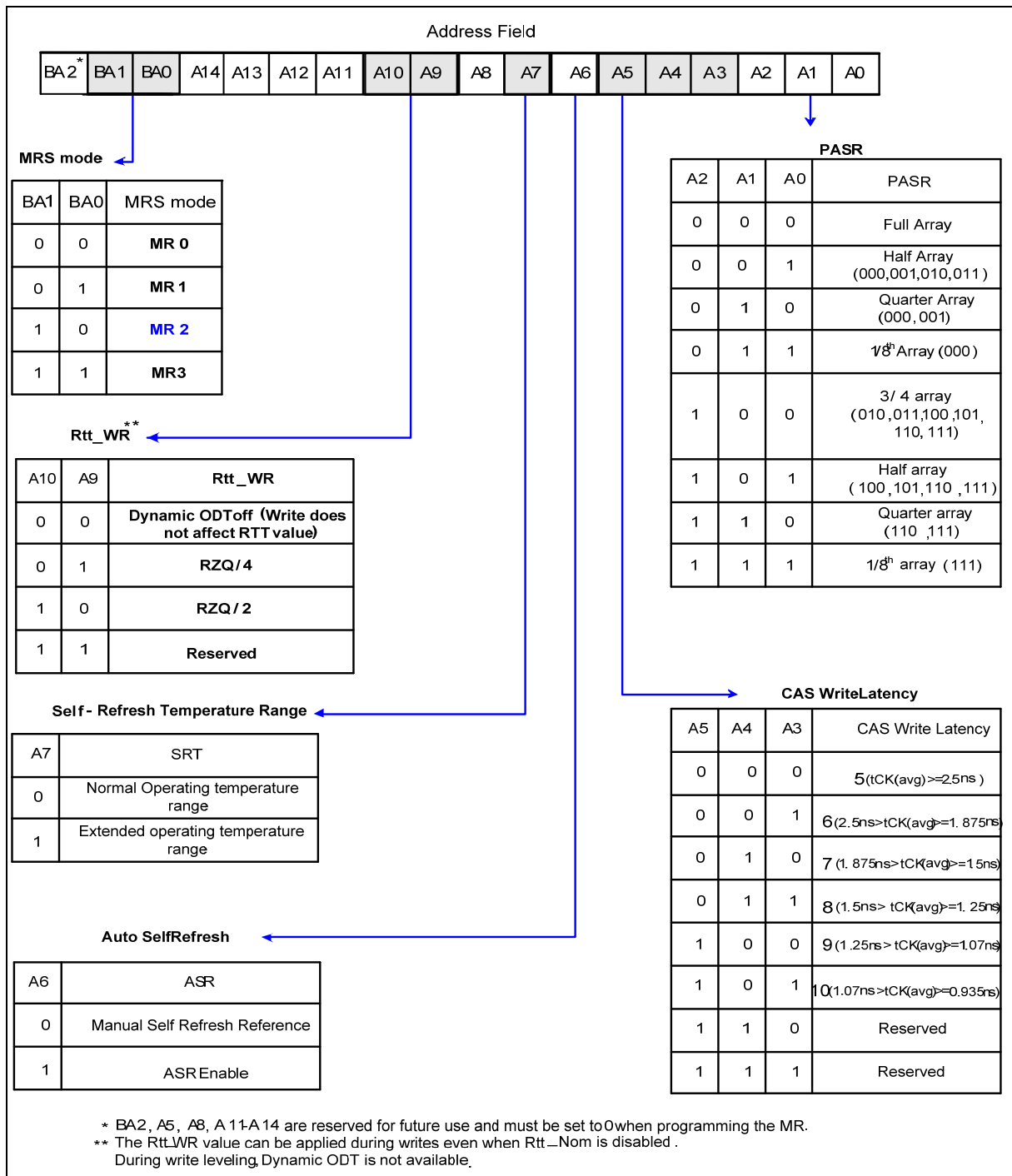
Fig. 7: MR2 Definition
