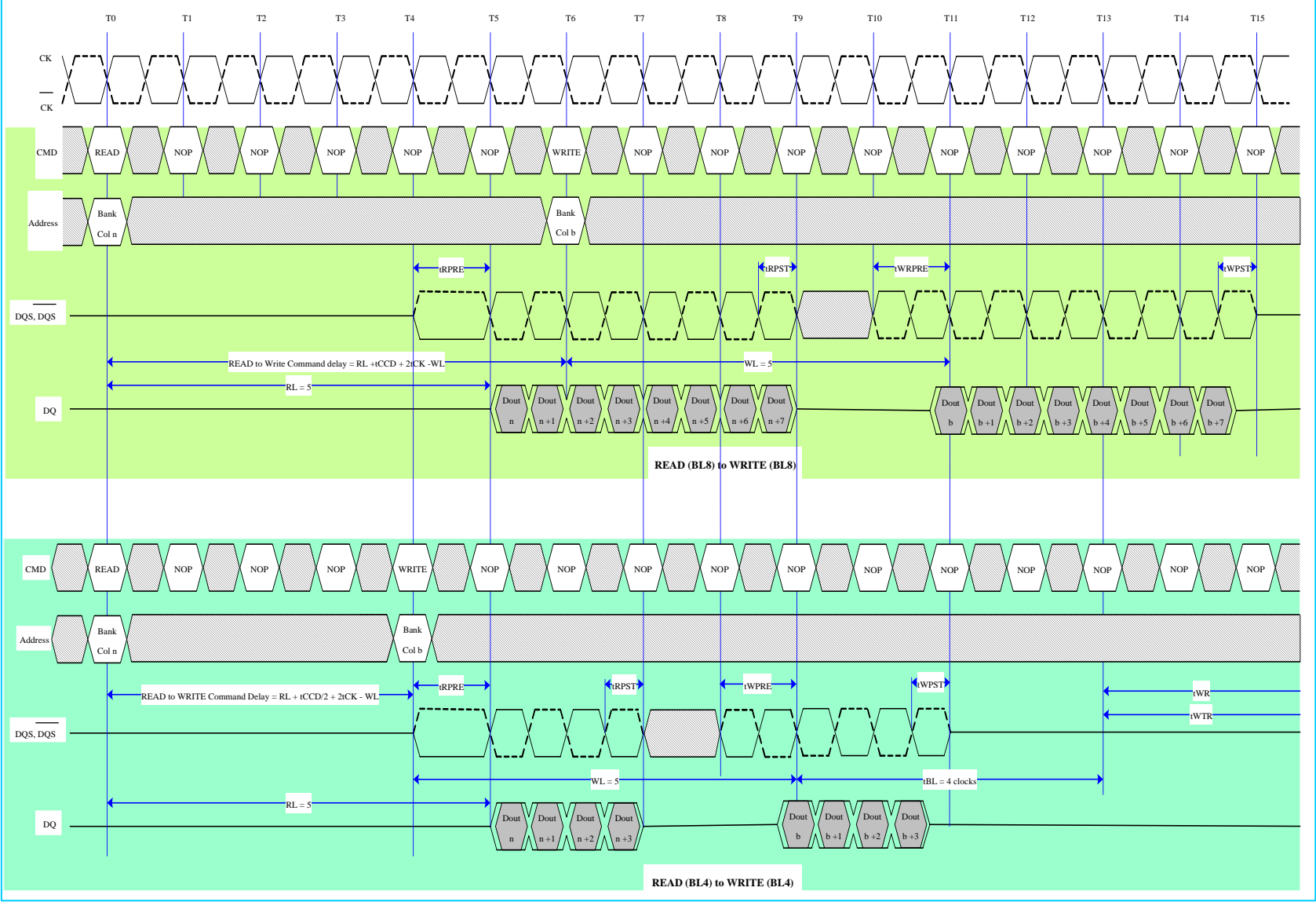
Fig. 23: READ to WRITE (CL=5, AL=0; CWL=5, AL=0)
