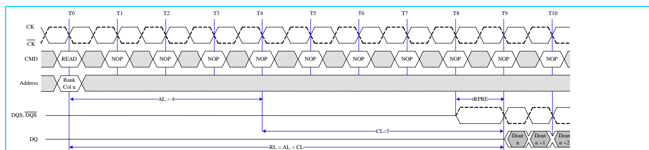
Fig. 18: READ Burst Operation RL = 9 (AL=4, CL=5, BL=8)
