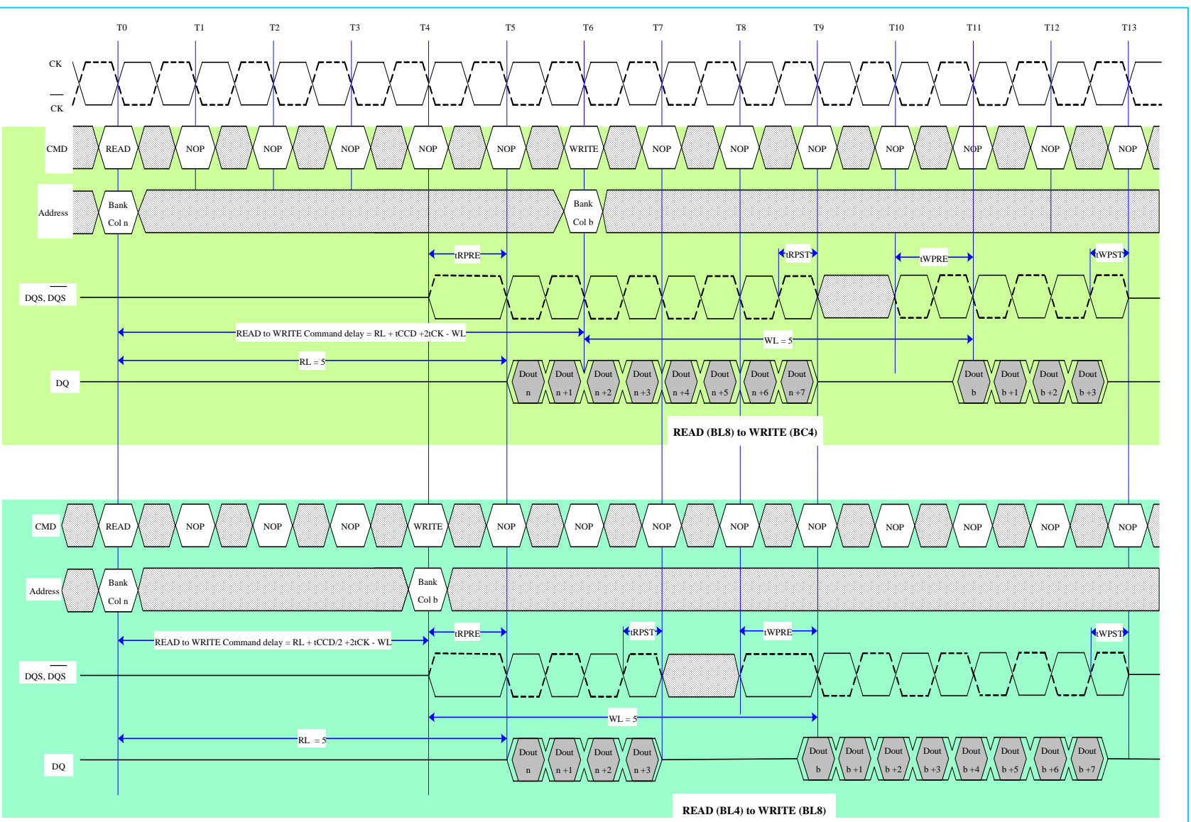
Fig. 25: READ to WRITE (CL=5, AL=0; CWL=5, AL=0)
