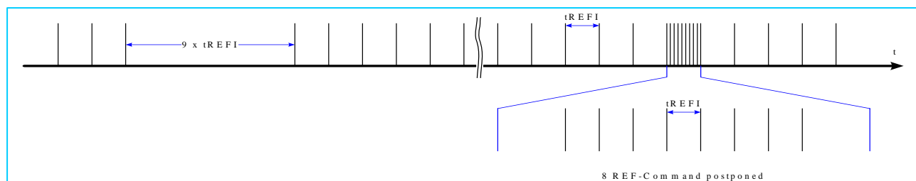
Fig. 31: Postponing Refresh Commands (Example)
