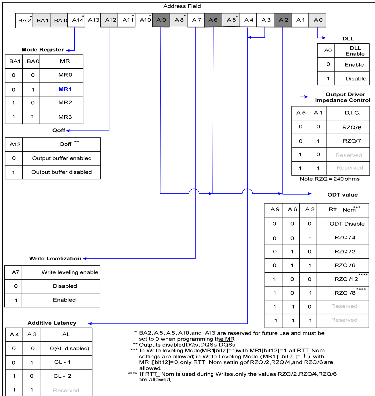
Fig. 6: MR1 Definition
