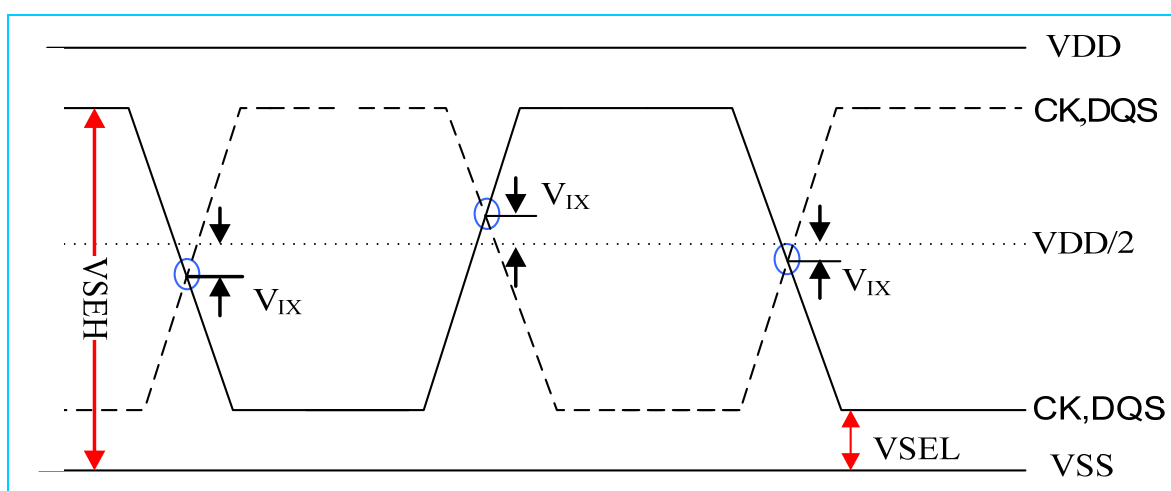
Fig. 60: Vix Definition
