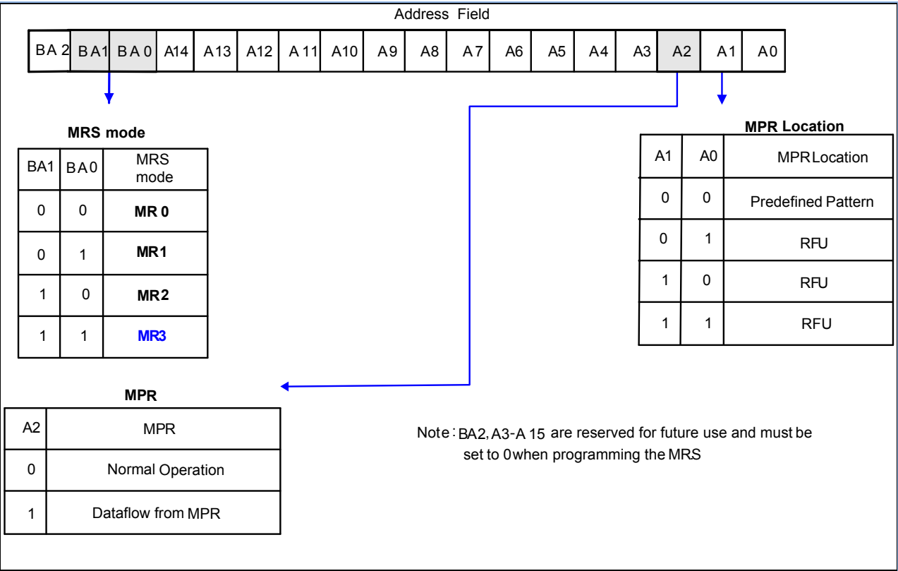
Fig. 8: MR3 Definition
