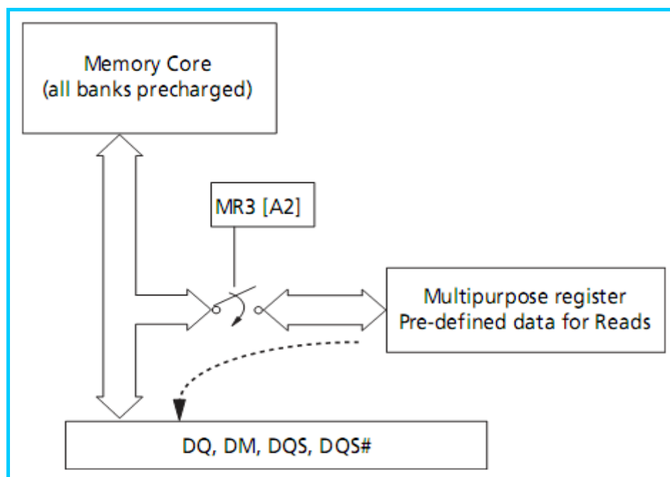
Fig. 9: MPR Block Diagram
