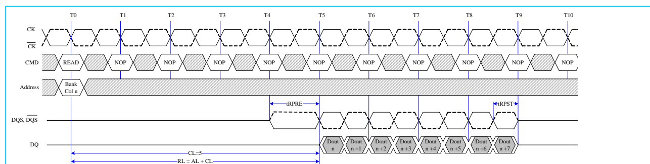
Fig. 17: Read Burst Operation RL=5 (AL=0, CL=5, BL=8)
