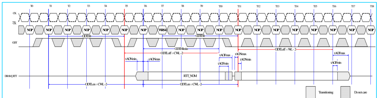
Fig. 46: Synchronous ODT example with BL=4, WL=7
