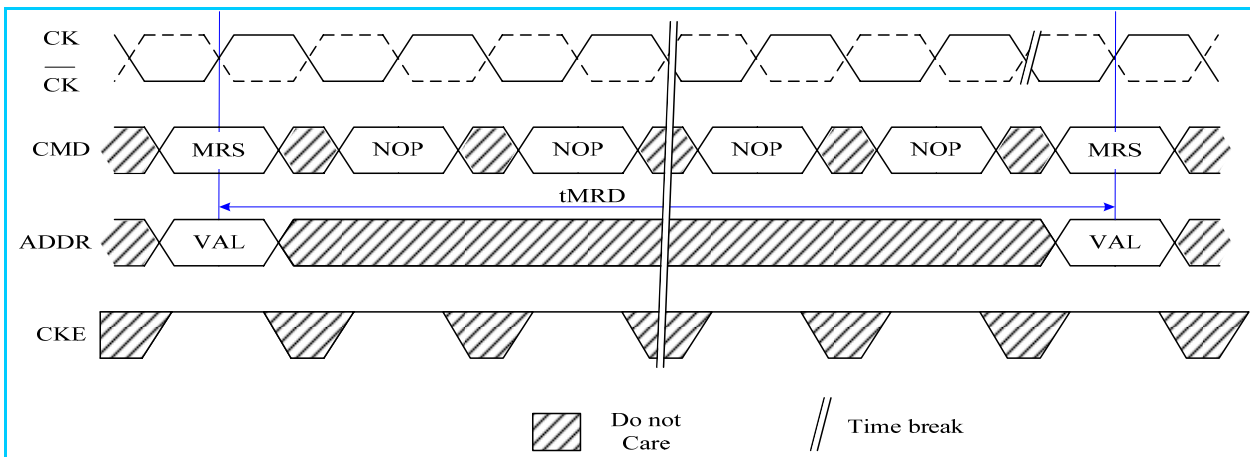
Fig. 3: t_{MRD} Timing
