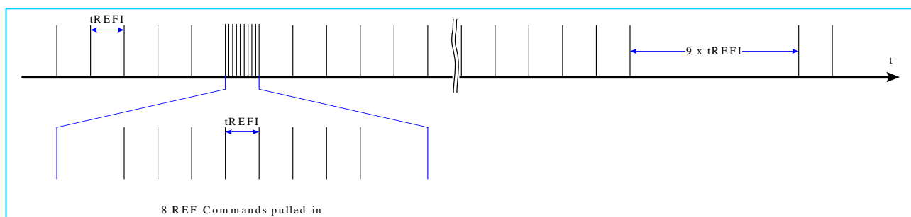
Fig. 32: Pulled-in Refresh Commands (Example)
