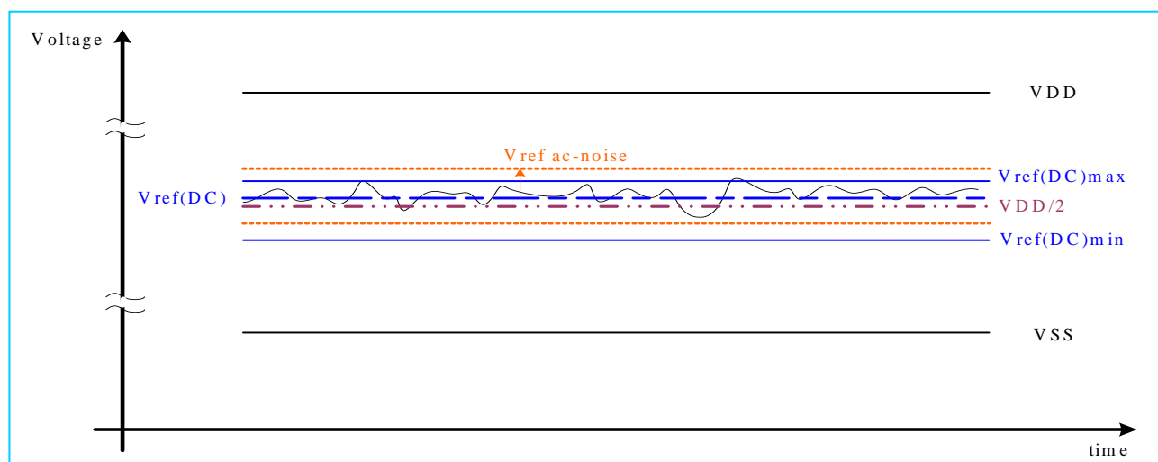
Fig. 58: Illustration of VREF(DC) tolerance and VREF ac-noise limits
