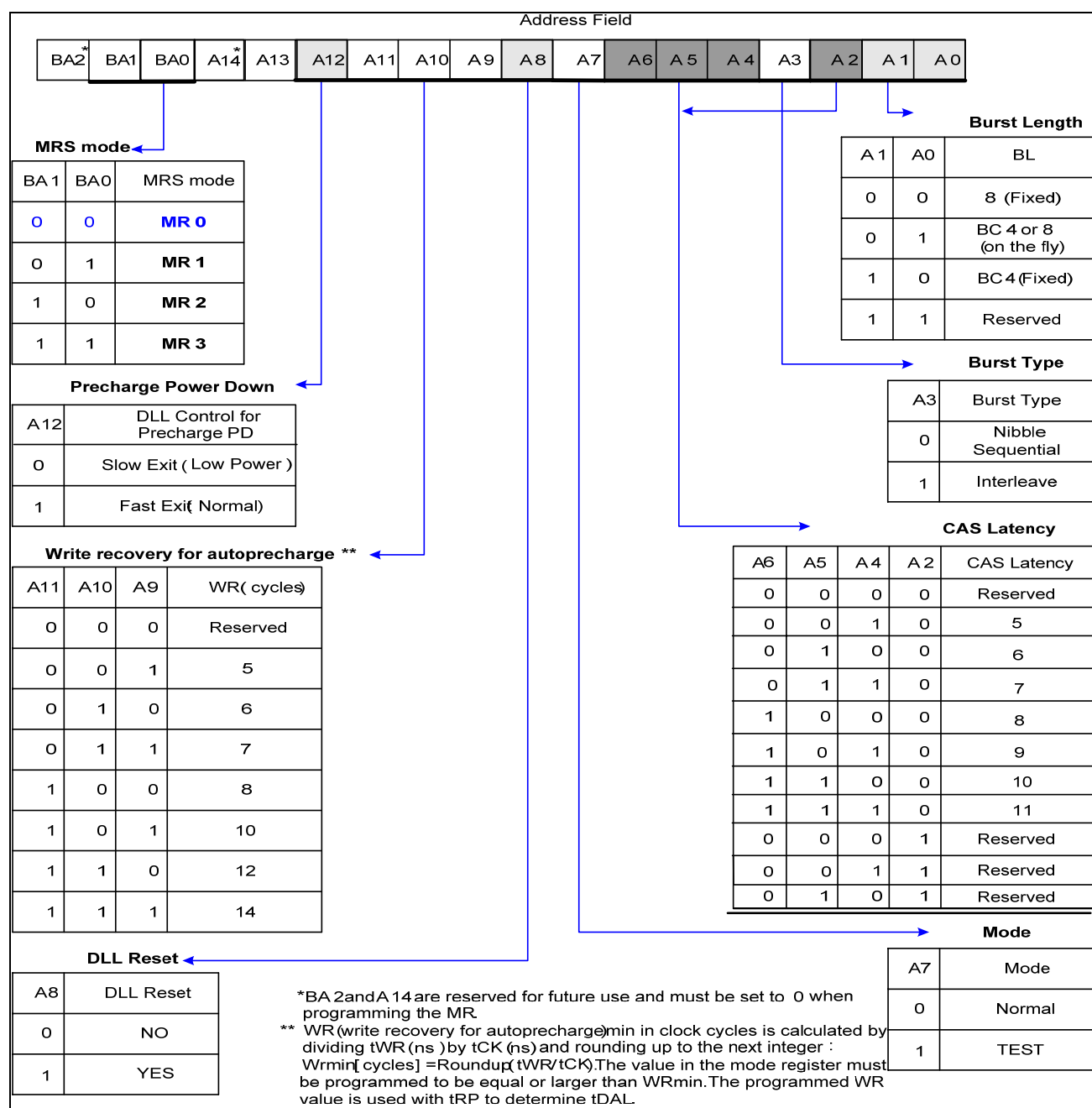
Fig. 5:MR0 Definition
