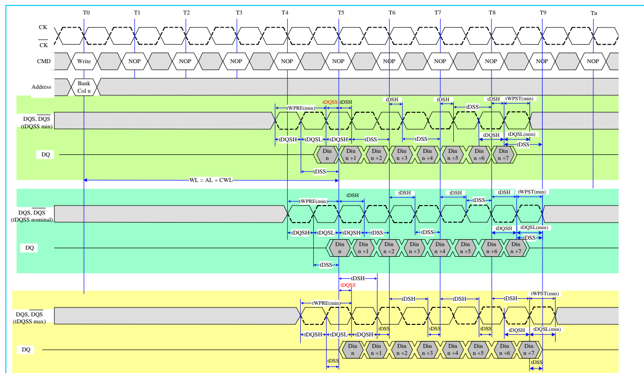
Fig. 26: Write Timing Definition
