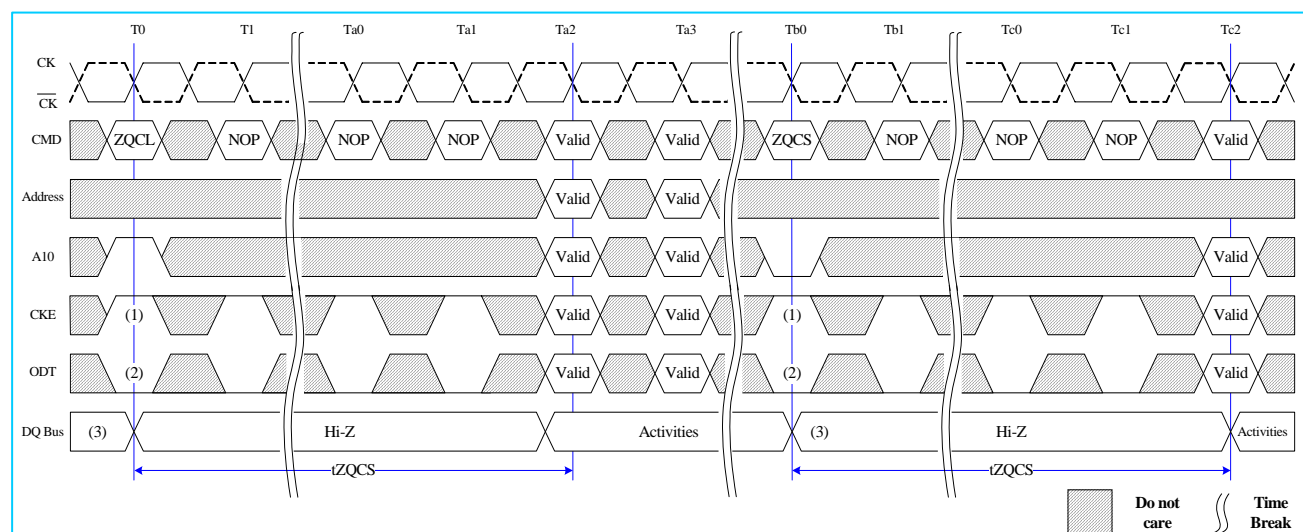
Fig. 57: ZQ Calibration Timing
