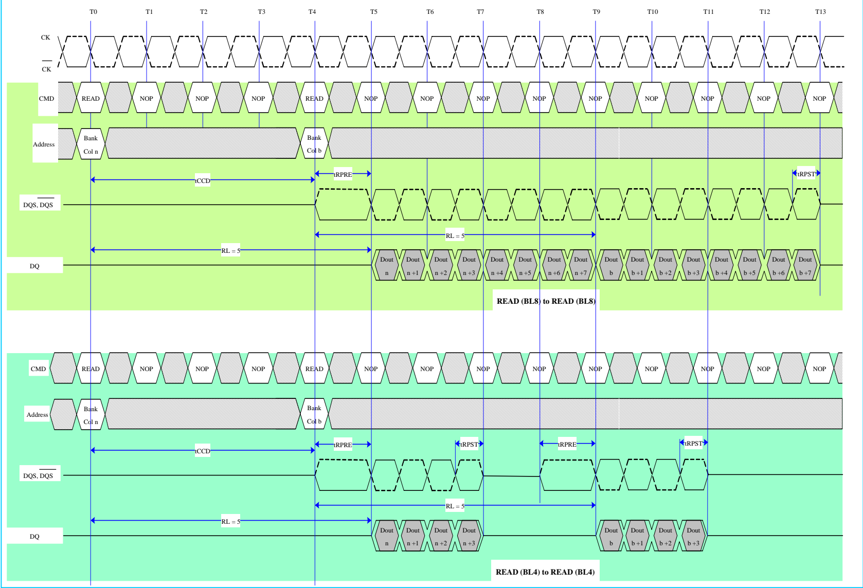
Fig. 22: Read to Read (CL=5, AL=0)
