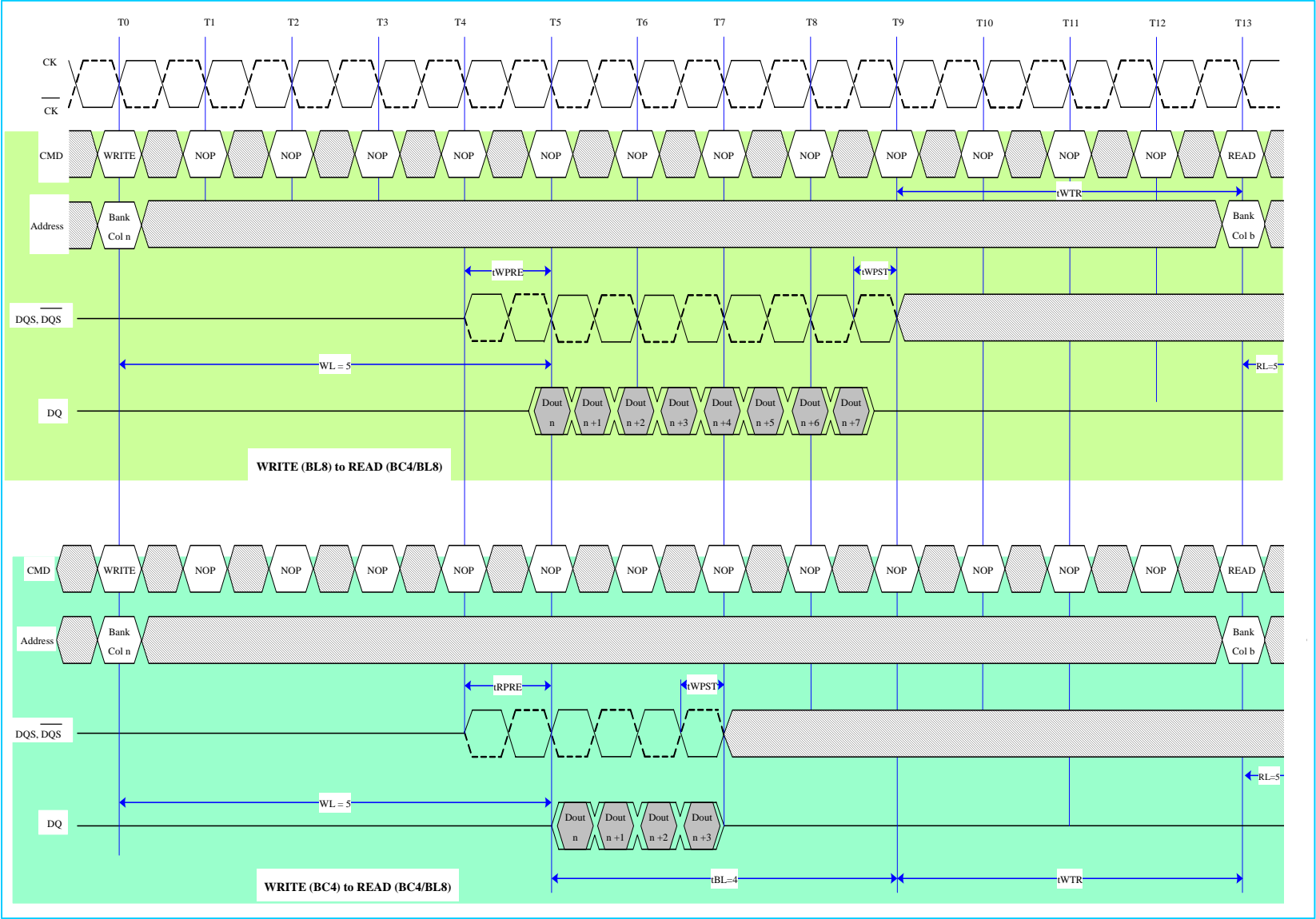
Fig. 28: WRITE to READ (RL=5, CL=5, AL=0; WL=5, CWL=5, AL=0; BL=4)
