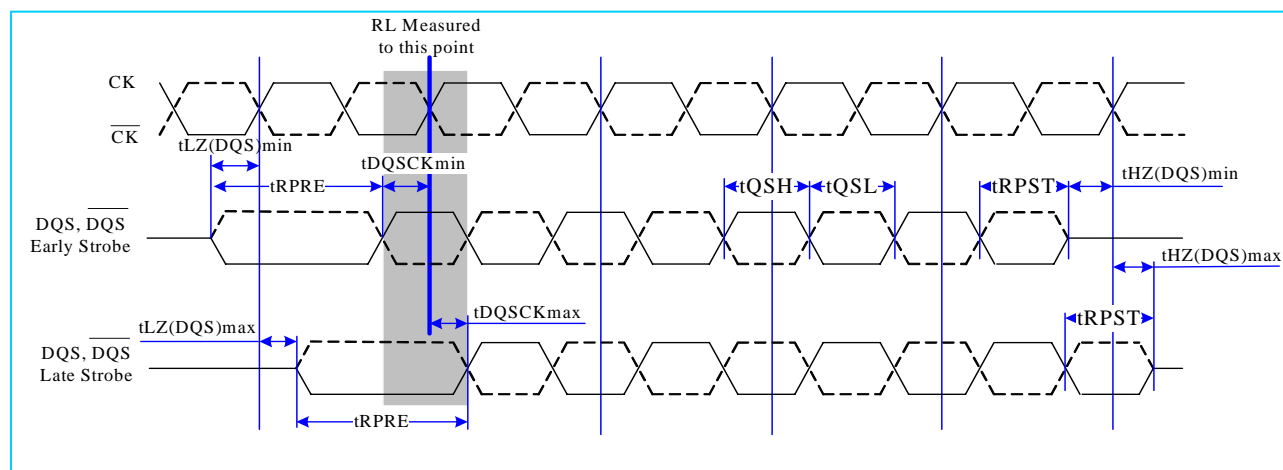
Fig. 20: Clock to Data Strobe Relationship
