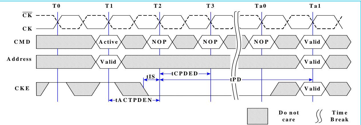
Fig. 41: Active Command to Power-Down Entry
