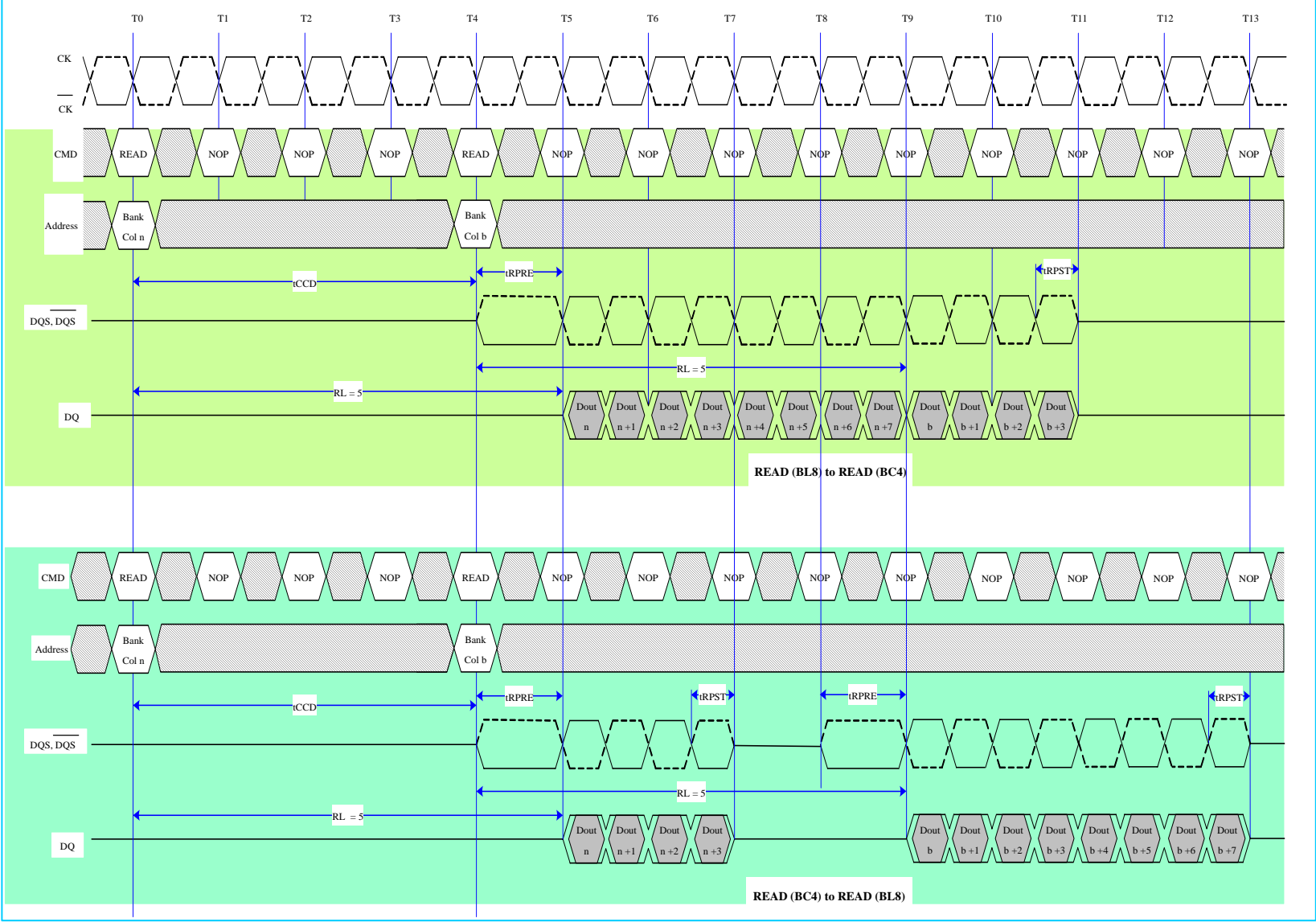
Fig. 24: READ to READ (CL=5, AL=0)
