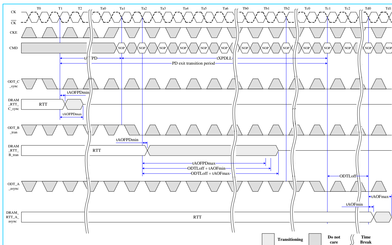
Fig. 55: Asynchronous to synchronous transition during Precharge Power Down (with DLL frozen) exit (CL=6; AL=CL-1; CWL=5; t_{ANPD}=WL-1=9 )
