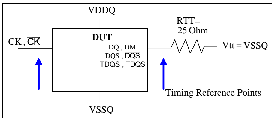
Fig. 66: ODT Timing Reference Load
