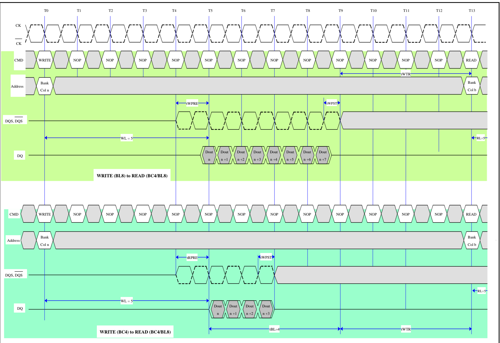
Fig. 28: WRITE to READ (RL=5, CL=5, AL=0; WL=5, AL=0; WL=5, CWL=5, AL=0; BL=4)
