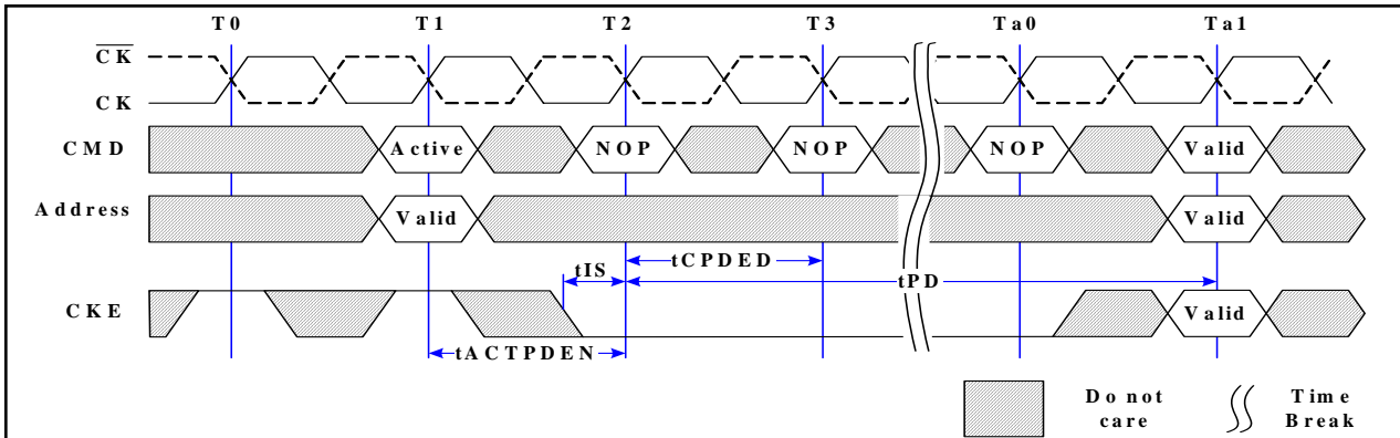
Fig. 41: Active Command to Power-Down Entry
