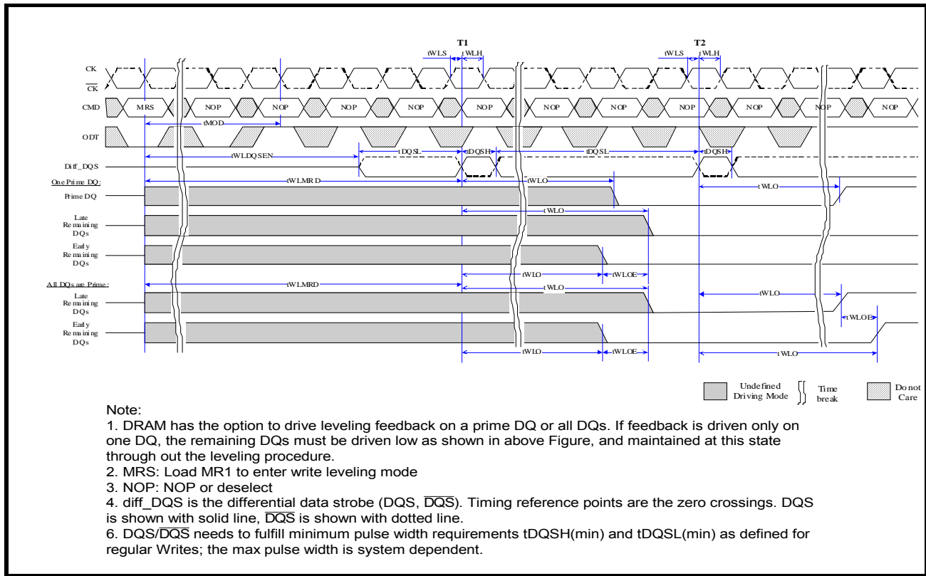
Fig. 15: Timing details of Write leveling sequence (DQS - \overline{DQS} is capturing CK - \overline{CK} low at T1 and CK - \overline{CK} high at T2)
