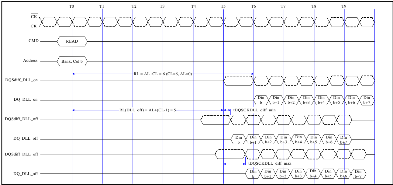
Fig. 10 DLL-off mode READ Timing Operation
