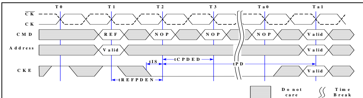
Fig. 40: Refresh Command to Power-Down Entry
