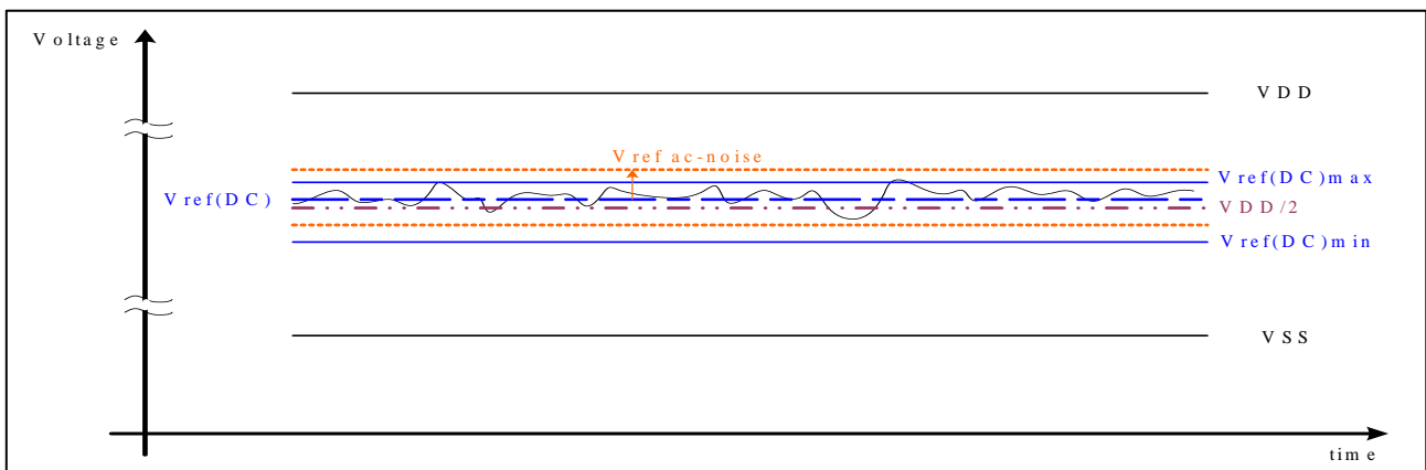
Fig. 58: Illustration of V_{ref}(DC) tolerance and V_{ref} ac-noise limits
