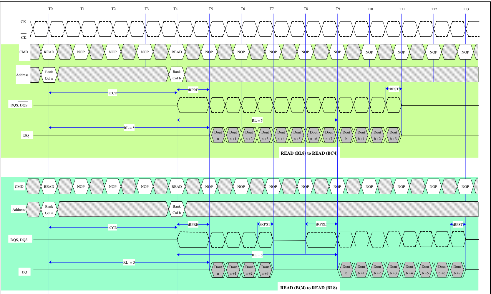
Fig. 24: READ to READ (CL=5, AL=0)
