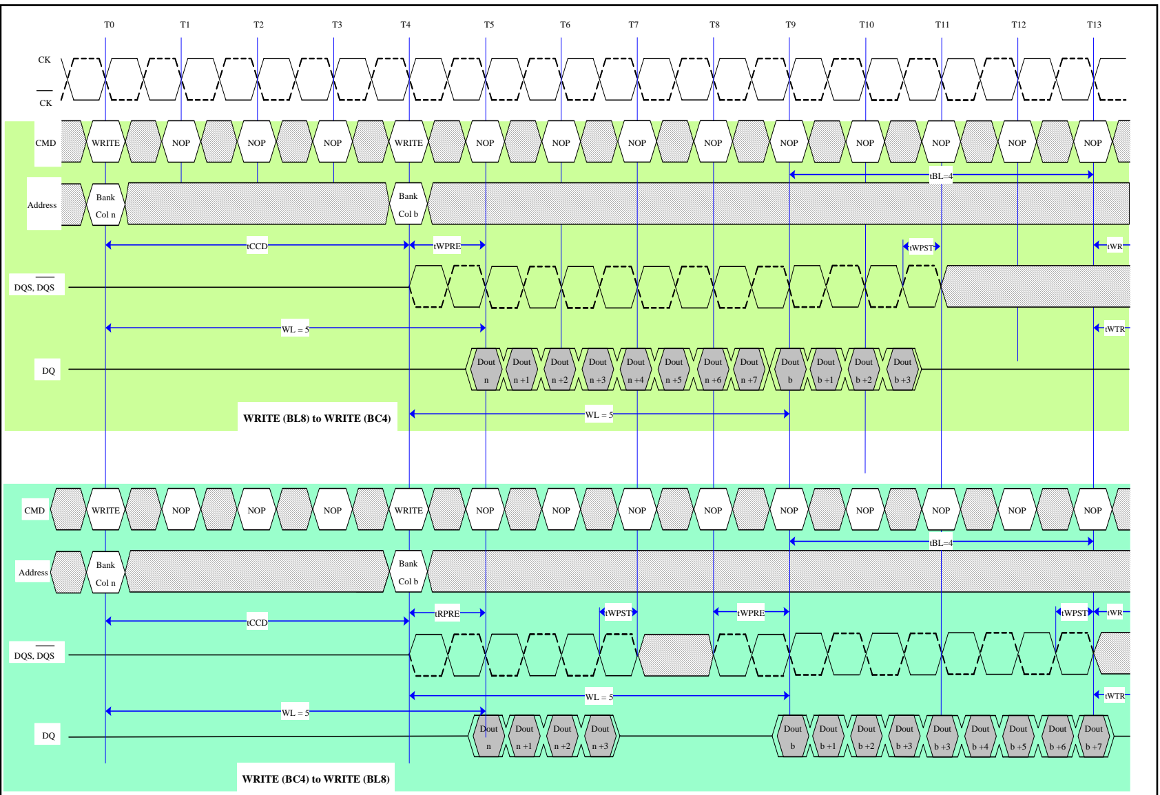
Fig. 29: WRITE to WRITE (WL=5, CWL=5, AL=0)
