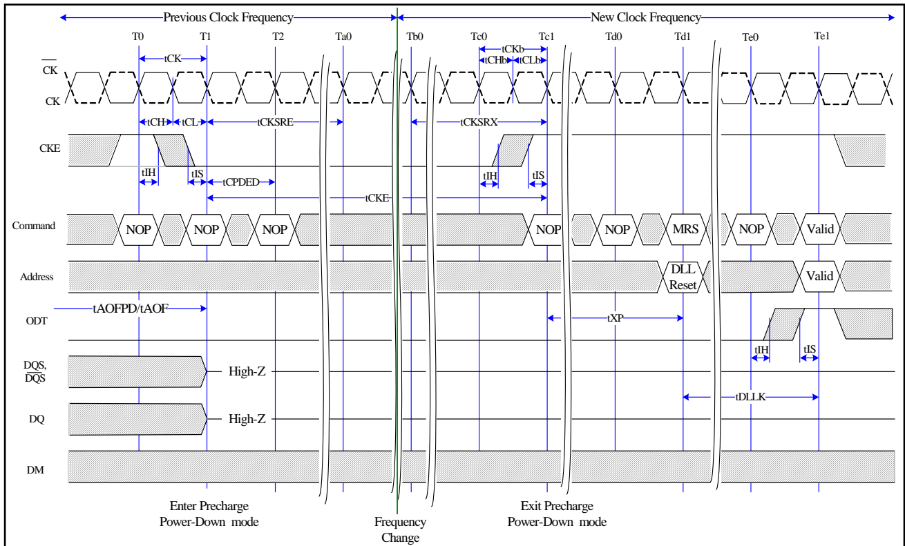
Fig. 13: Change Frequency during Precharge Power-down
