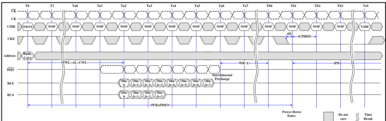
Fig. 36: Power-Down Entry after Write with Auto Precharge
