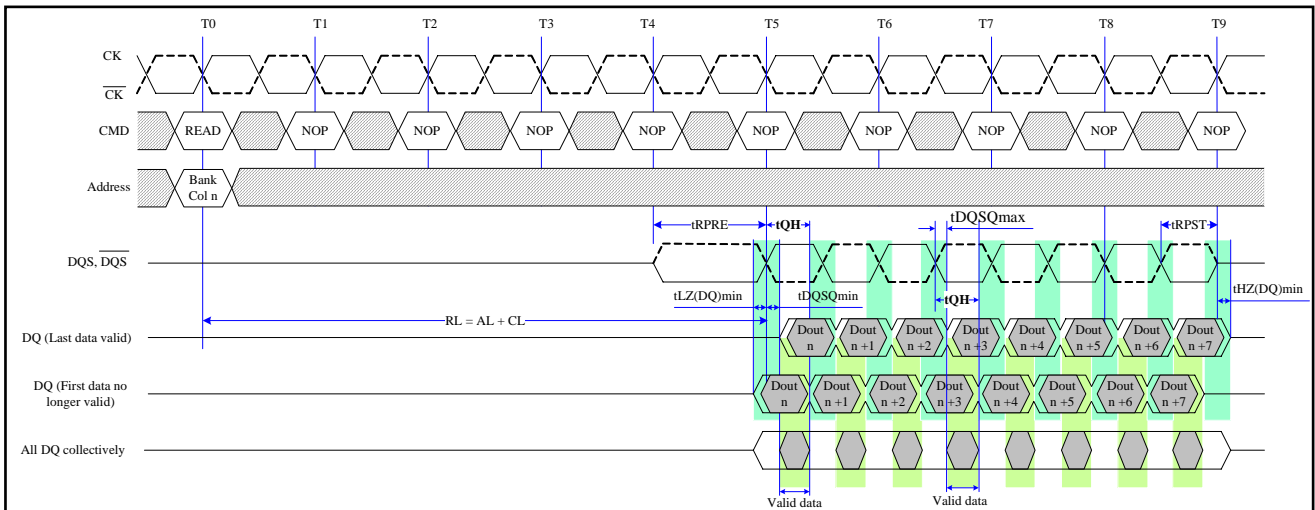
Fig. 21: Data Strobe to Data Relationship
