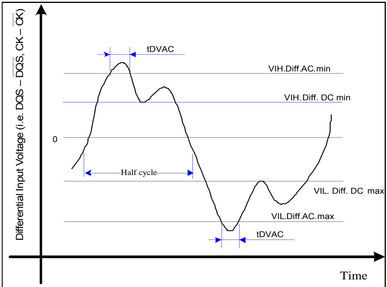
Fig. 59: Definition of differential ac-swing and “time above ac-level”
