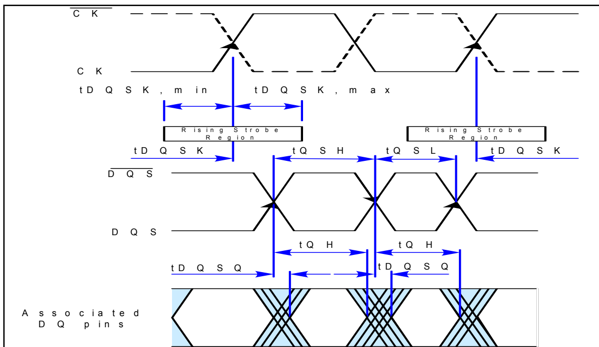
Fig. 19: Read Timing Definition
