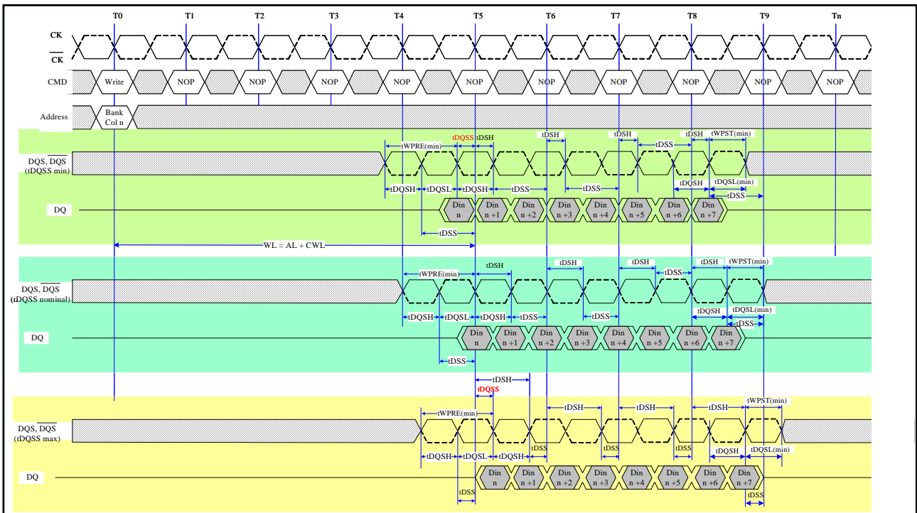
Fig. 26: Write Timing Definition
