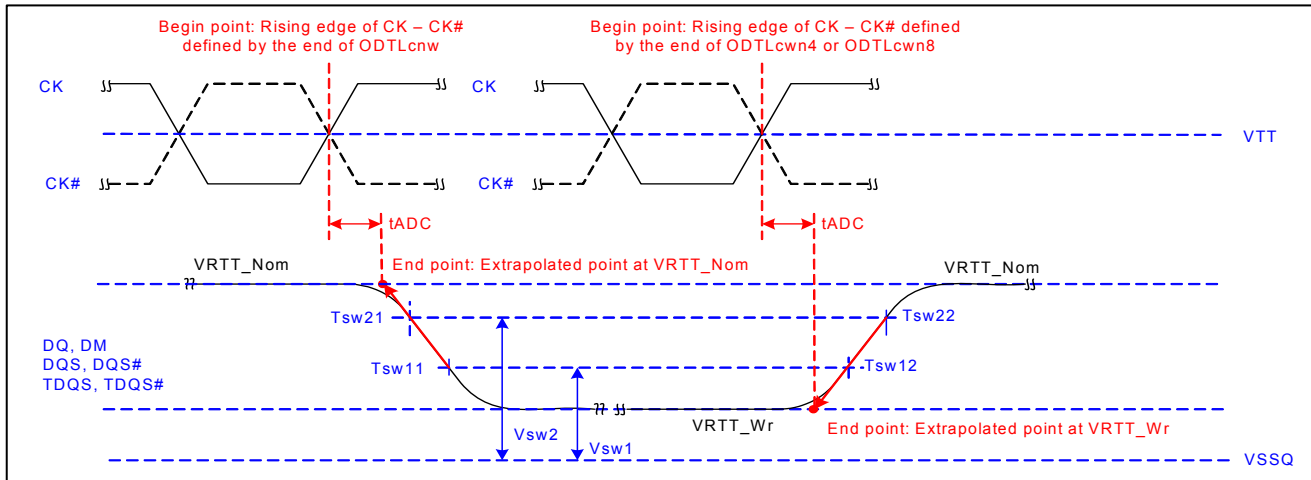
Fig. 71: Definition of t_{ADC}
