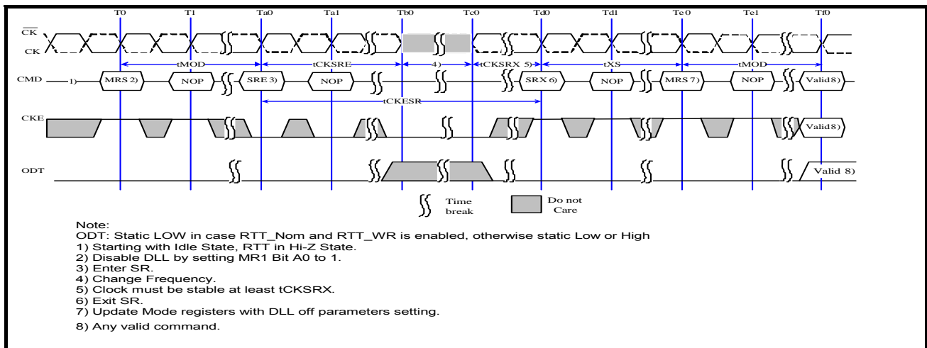
Fig. 11: DLL Switch Sequence from DLL-on to DLL-off
