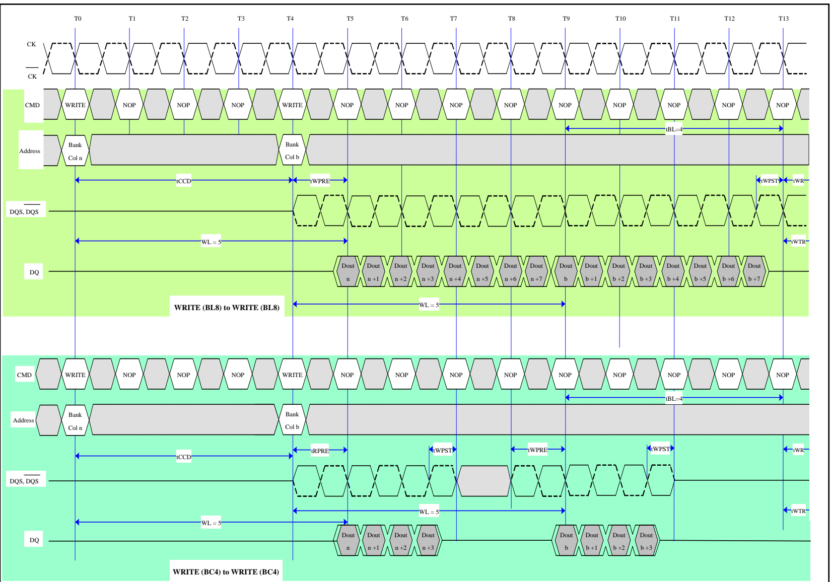
Fig. 27: WRITE to WRITE (WL=5; CWL=5, AL=0)
