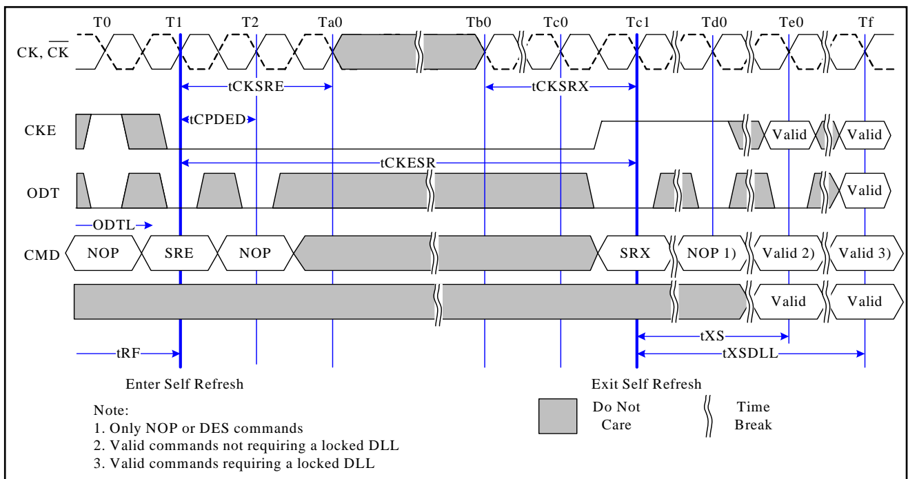
Fig. 33: Self-Refresh Entry/Exit Timing
