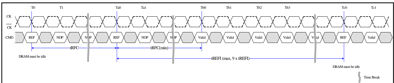
Fig. 31: Postponing Refresh Commands (Example)
