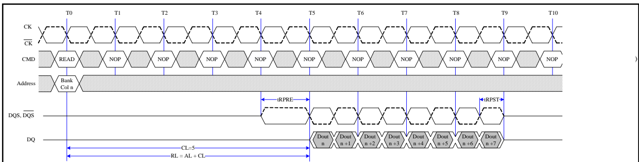
Fig. 17: Read Burst Operation RL=5 (AL=0, CL=5, BL=8)
