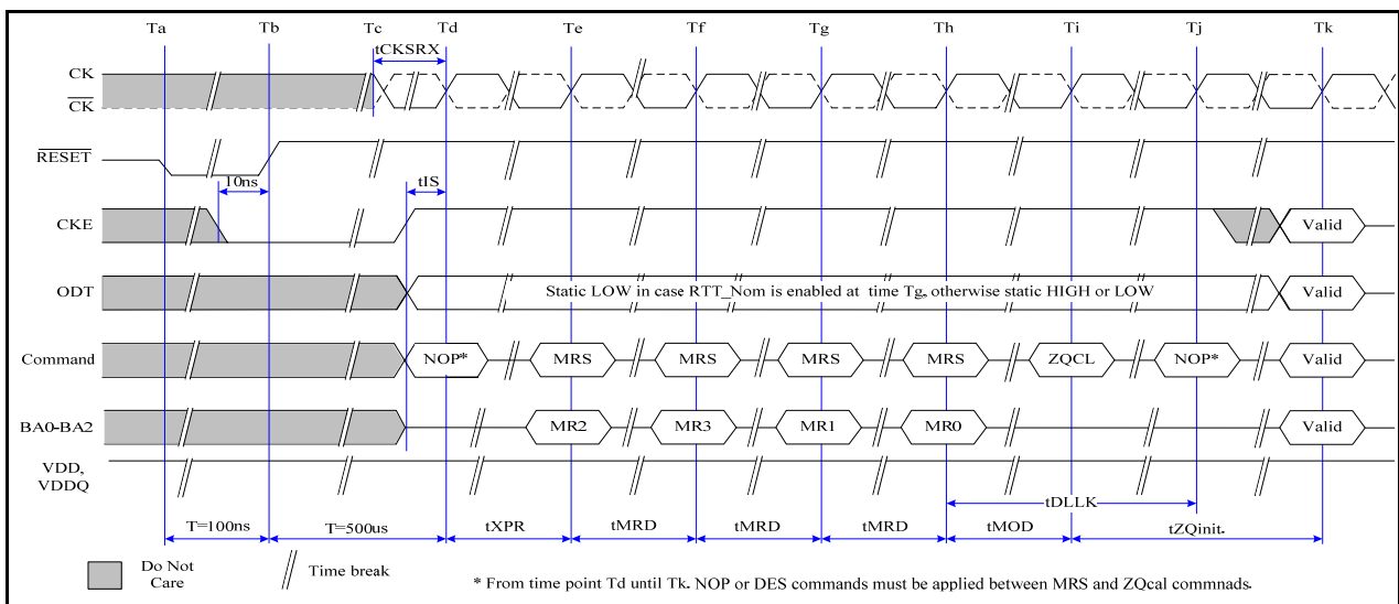
Fig. 2: Reset Procedure at Power Stable Condition
