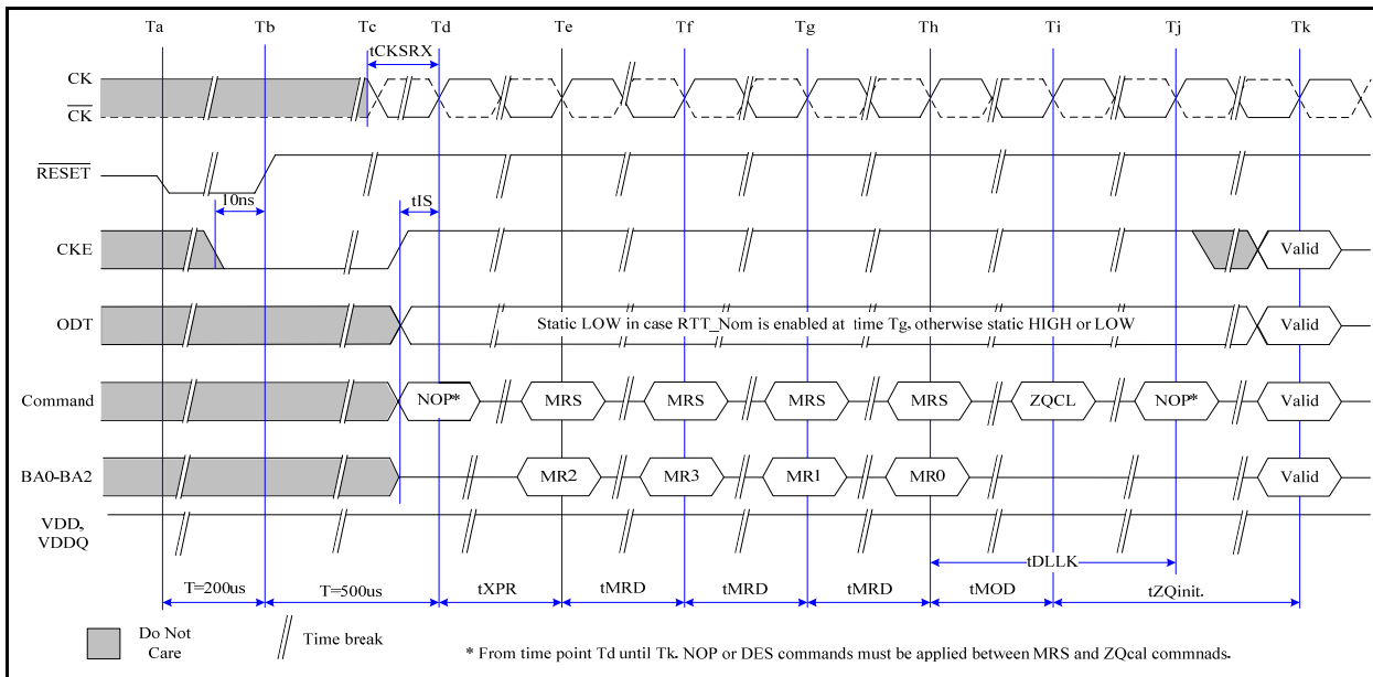
Fig. 1: Reset and Initialization Sequence at Power- on Ramping (Cont'd)
