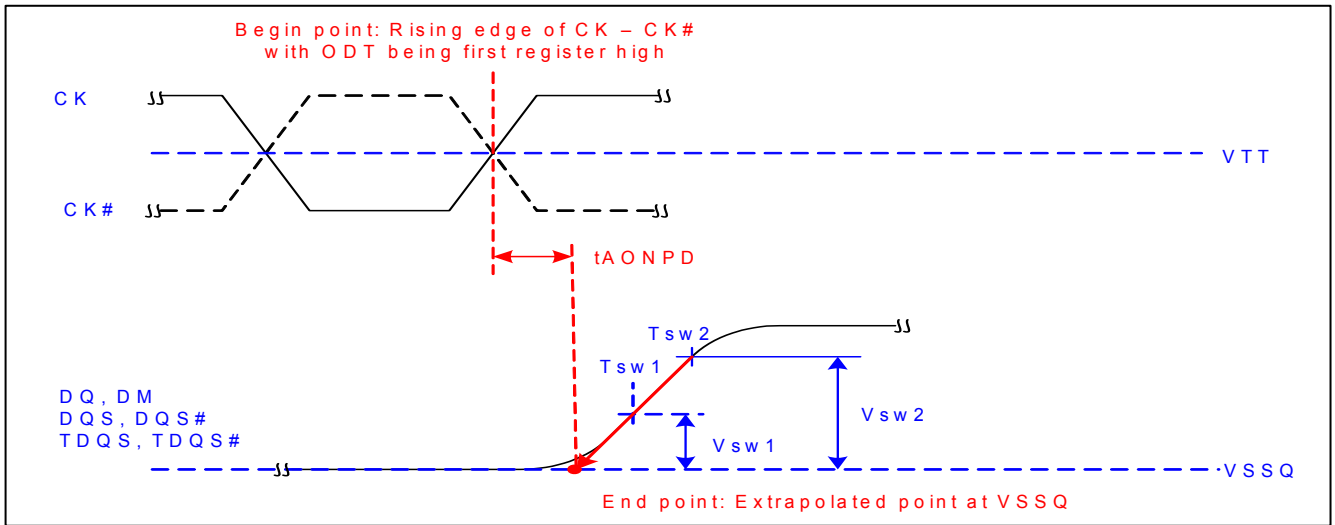
Fig. 69: Definition of t_{AOF}
