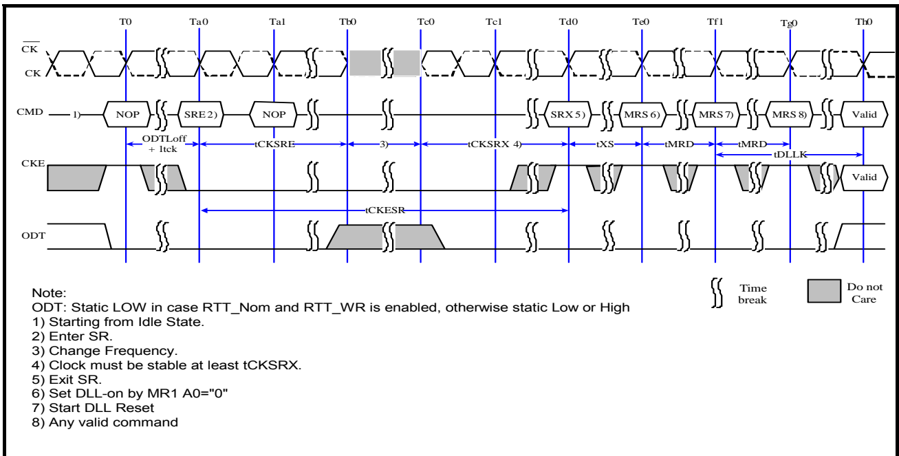
Fig. 12 DLL Switch Sequence from DLL-on to DLL-off
