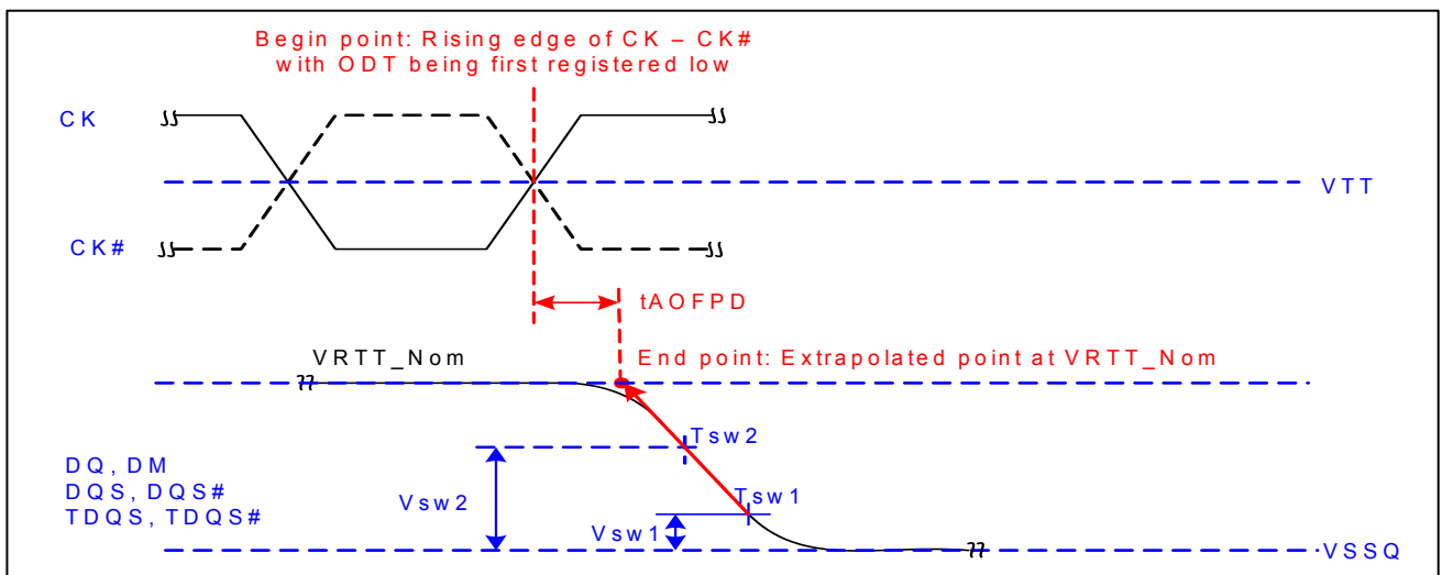
Fig. 70: Definition of t_{AOFPD}
