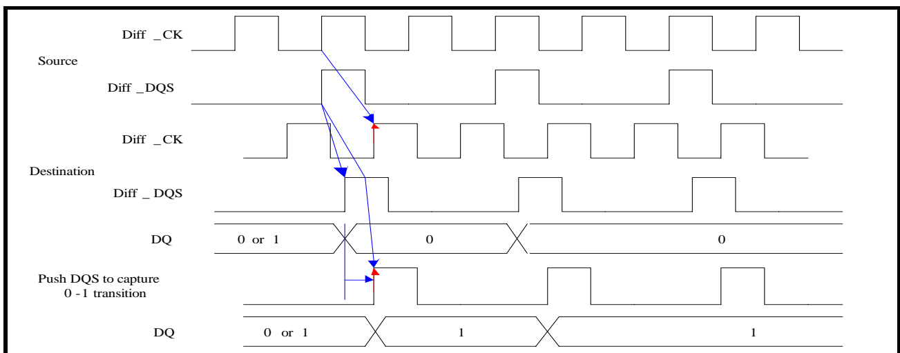
Fig. 14: Write Leveling Concept
