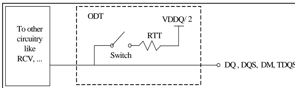
Fig. 44: Functional Representation of ODT
