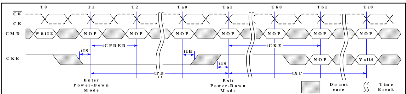
Fig. 38: Precharge Power-Down (Fast Exit Mode) Entry and Exit
