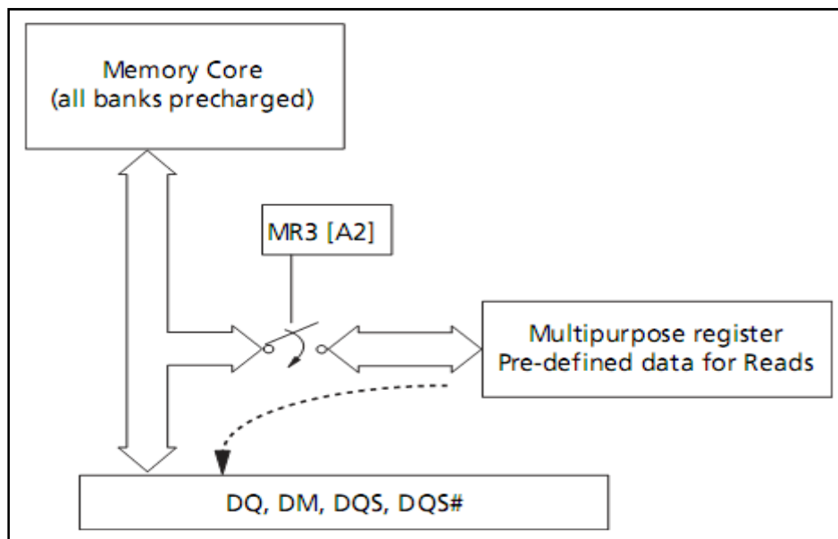
Fig. 9: MPR Block Diagram
