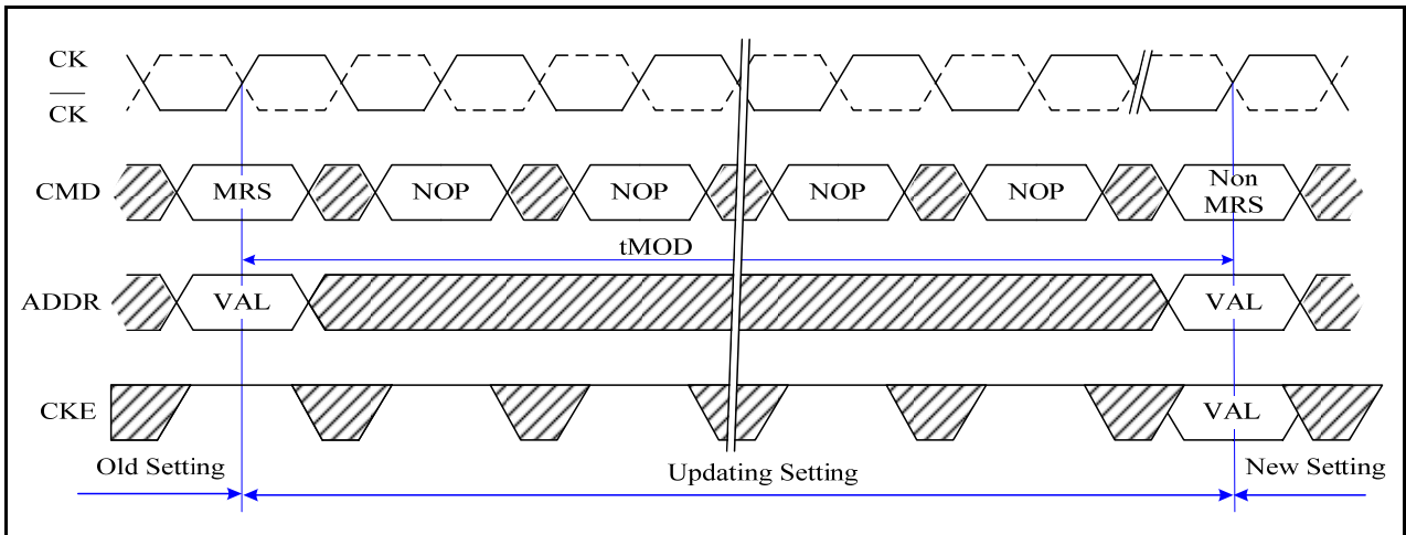
Fig. 4: t MOD Timing
