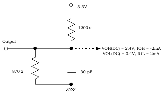
(Fig.1) DC Output Load circuit
