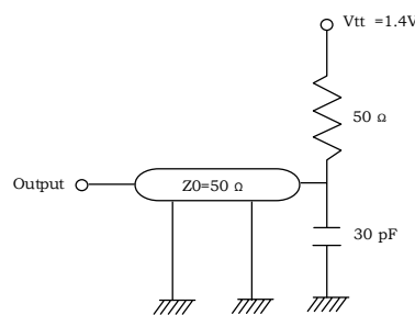
(Fig.2) AC Output Load Circuit
