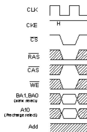
Fig. 3 Precharge command
