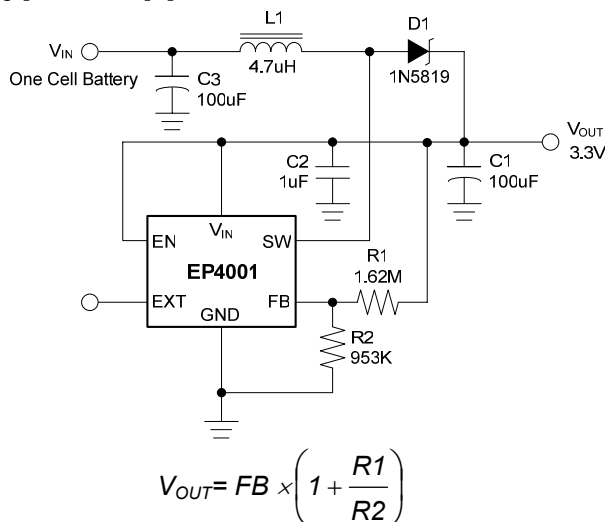
Figure 1-Basic application circuit with EP4001
