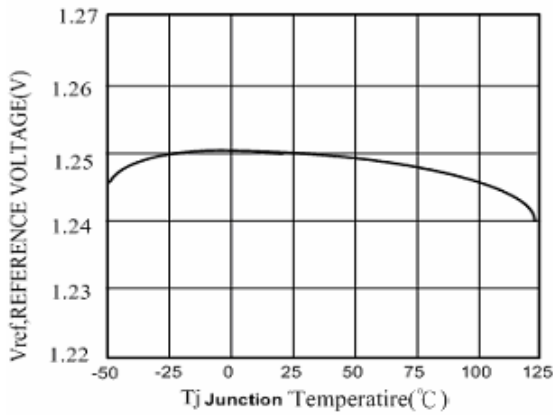
Figure 9. Temperature Stability
