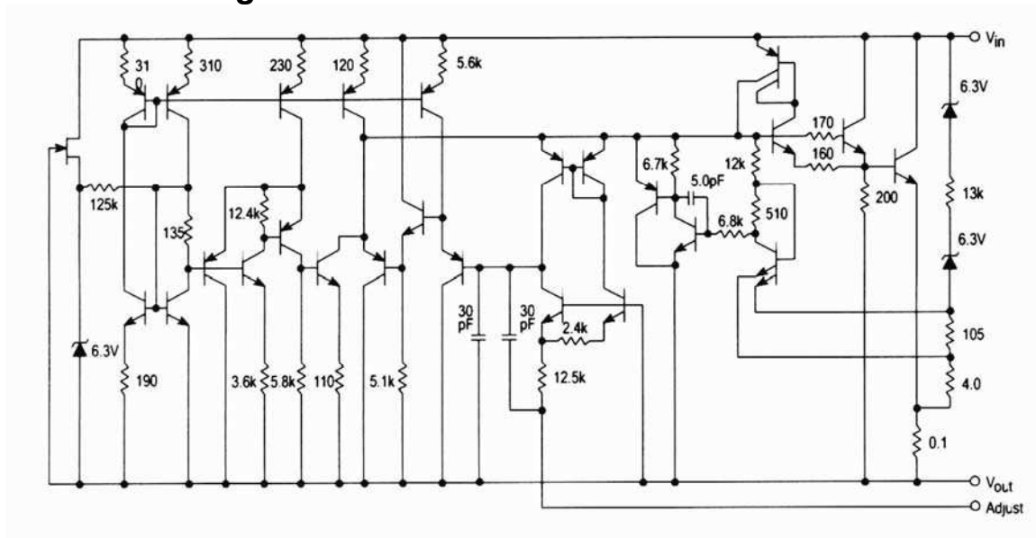
EP1017 contains 29 active transistors
