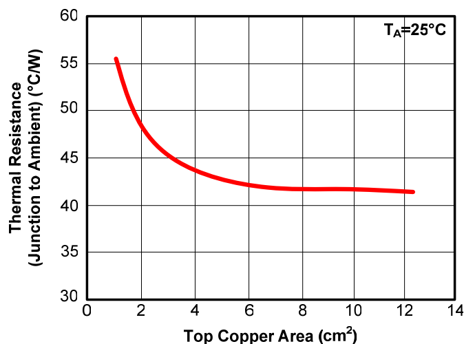
Figure 3- \theta_{(JA)} vs copper area for SOT-223 package
