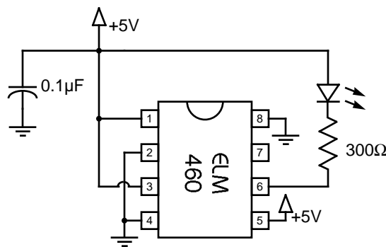
Figure 3. LED Flasher
