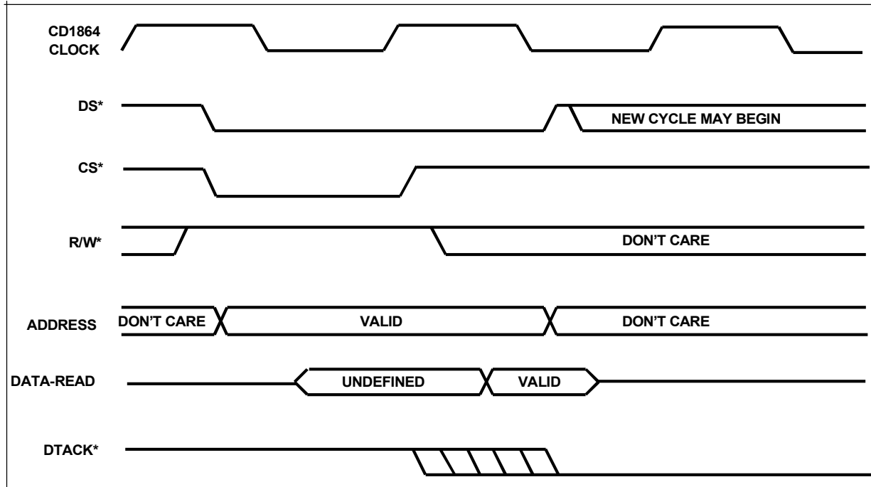
Figure 18. Typical Clocked Bus Interface
