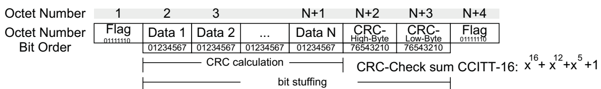
Figure 20: HDLC frame format
