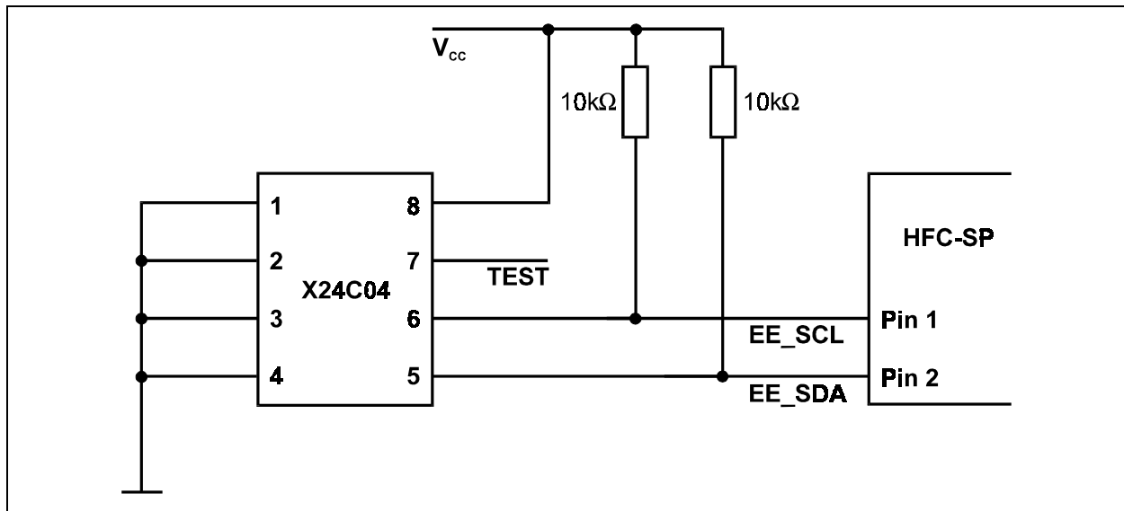
Figure 11: EEPROM circuitry
