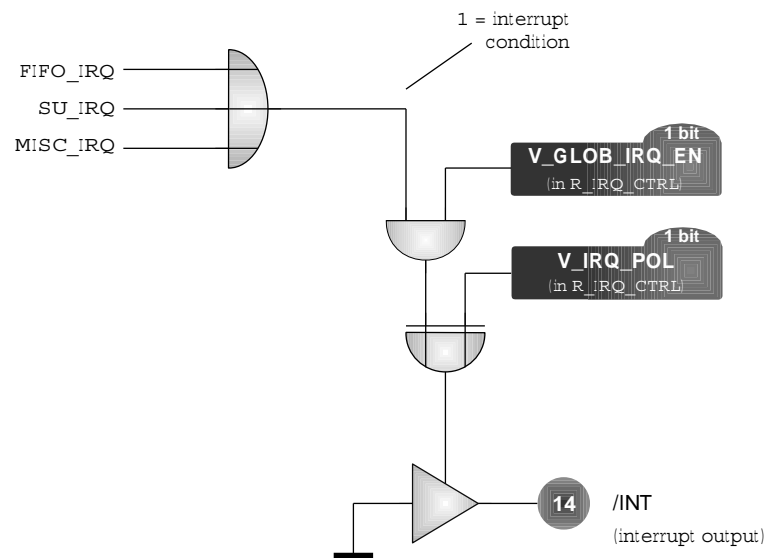
Figure 9.5: Interrupt output
