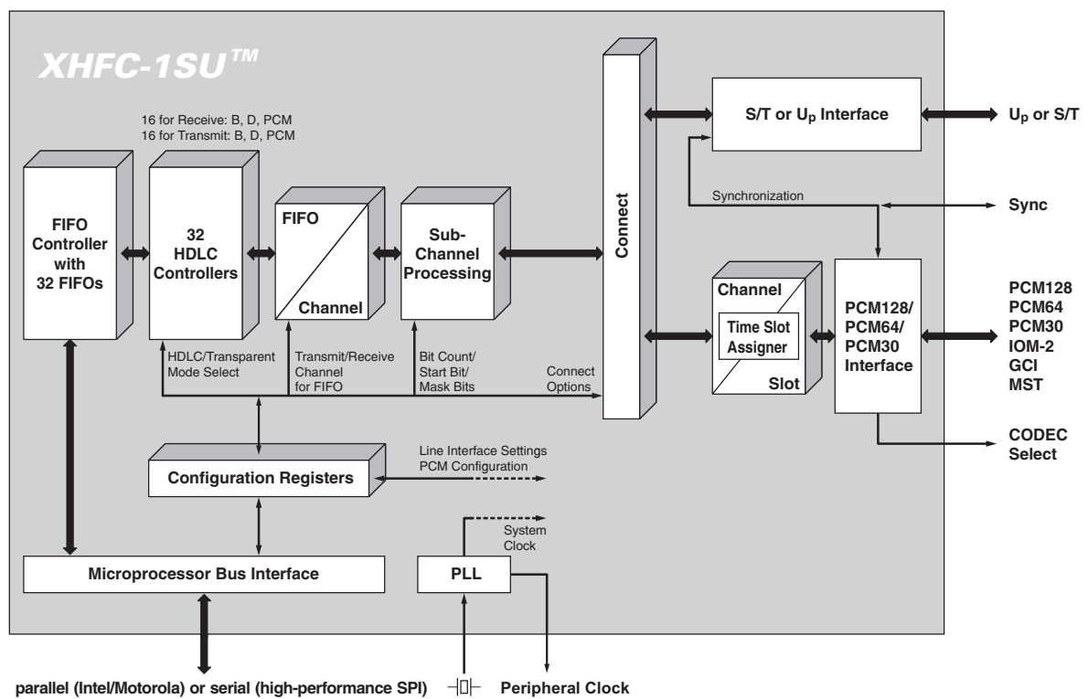
Figure 1.1: XHFC-1SU block diagram
