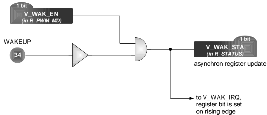
Figure 9.10: Wakeup interrupt
