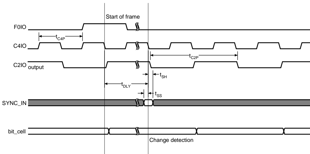
Figure 6.11: Timing specification of the SYNC_IN change detection
