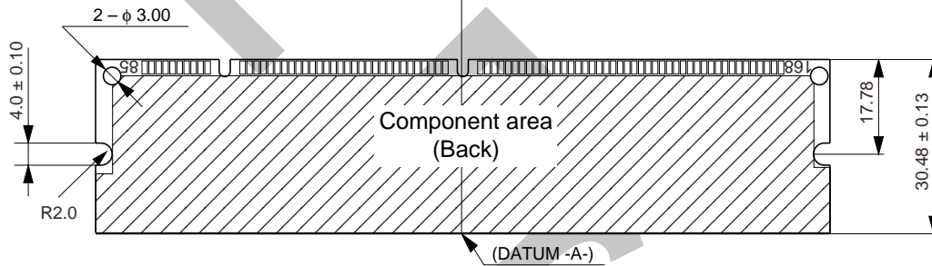
Detail A
