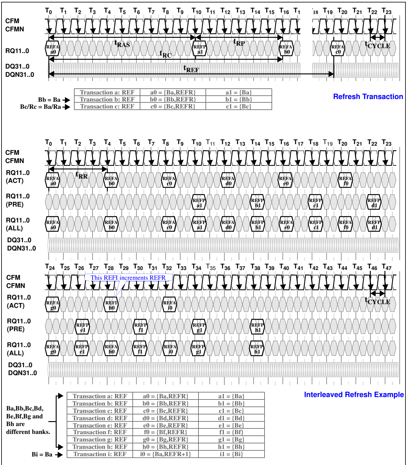
Figure 34 Refresh Transactions
