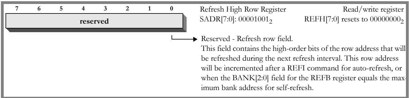
Figure 23 Refresh High (REFH) Row Register
