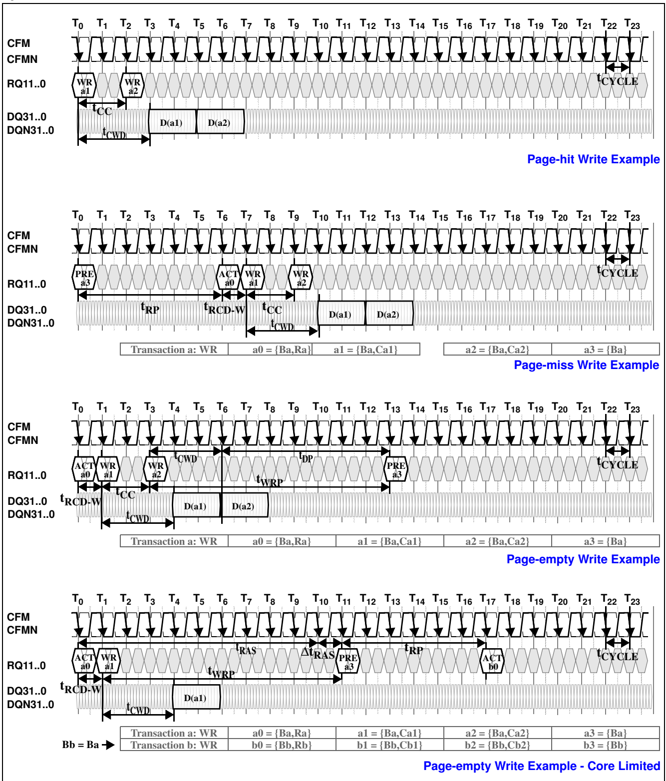
Figure 8 Write Transactions
