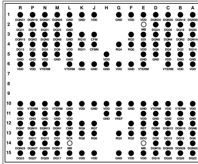
Top view of package
