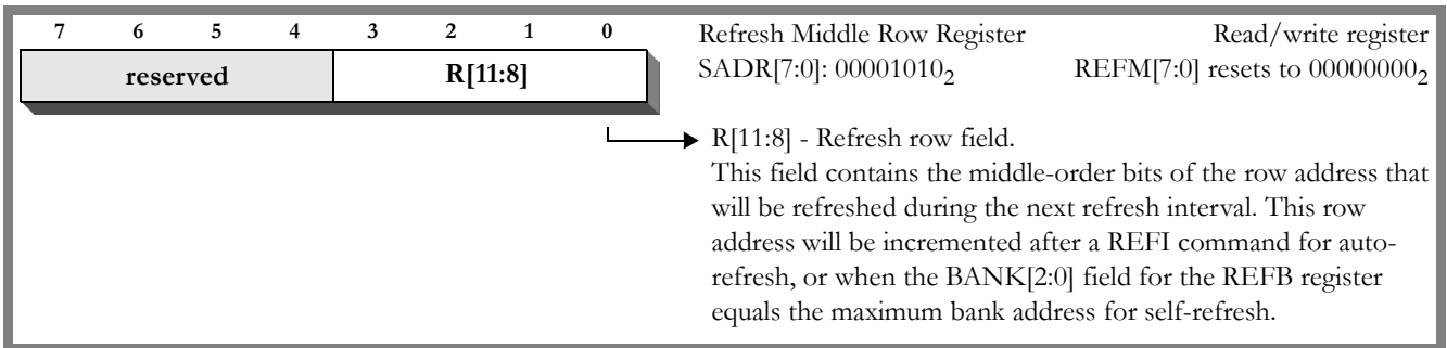
Figure 24 Refresh Middle (REFM) Row Register
