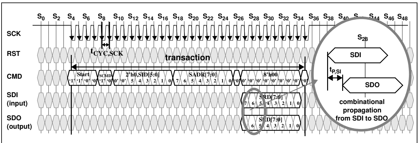
Figure 15 Serial Read Transaction — Non-selected DRAM
