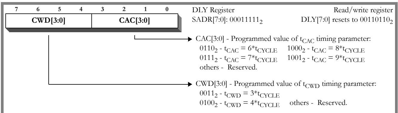
Figure 33 Delay (DLY) Control Register
