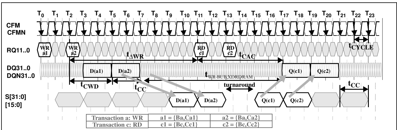
Figure 44 Write/Read Interaction — ERAW Feature
