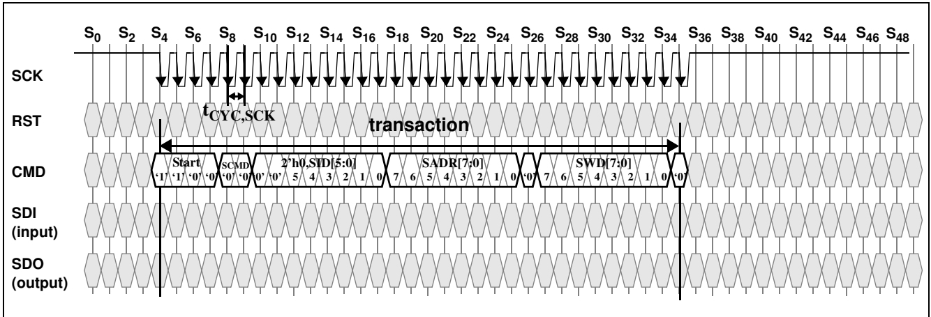
Figure 13 Serial Write Transaction
