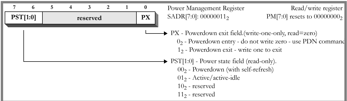
Figure 18 Power Management (PM) Register
