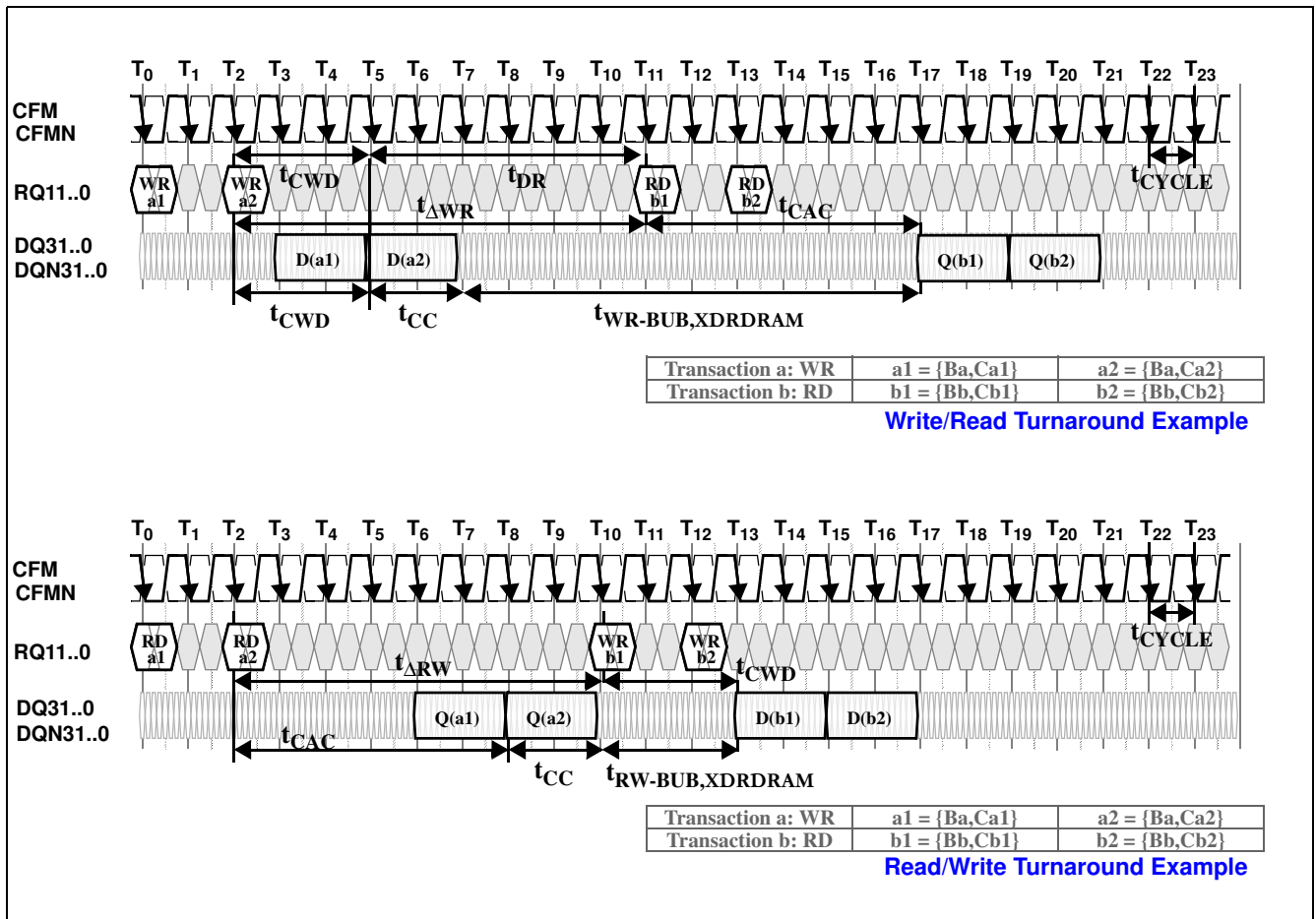
Figure 11 Write/Read Interaction
