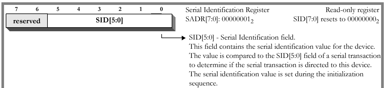
Figure 16 Serial Identification (SID) Register
