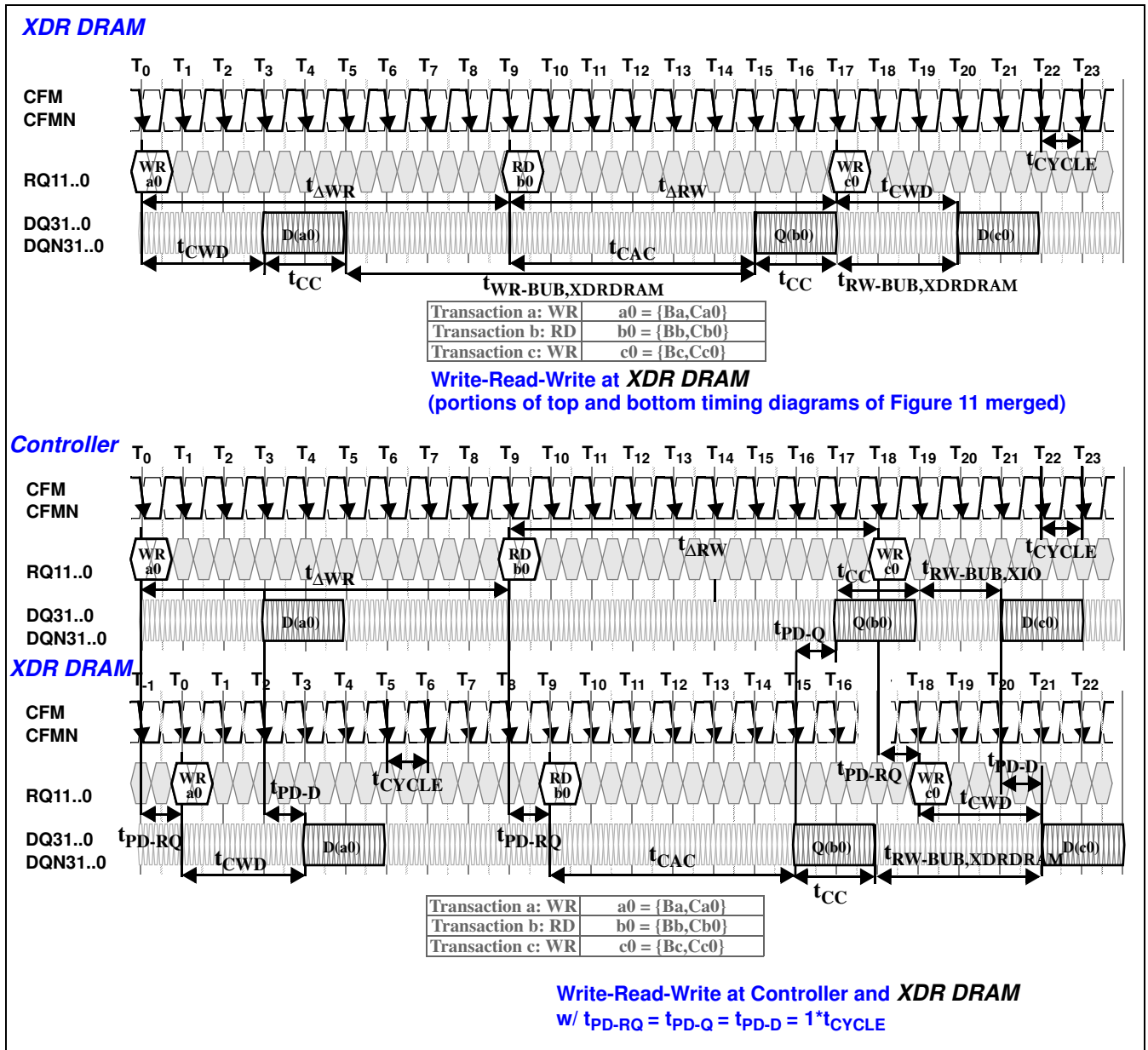
Figure 12 Propagation Delay
