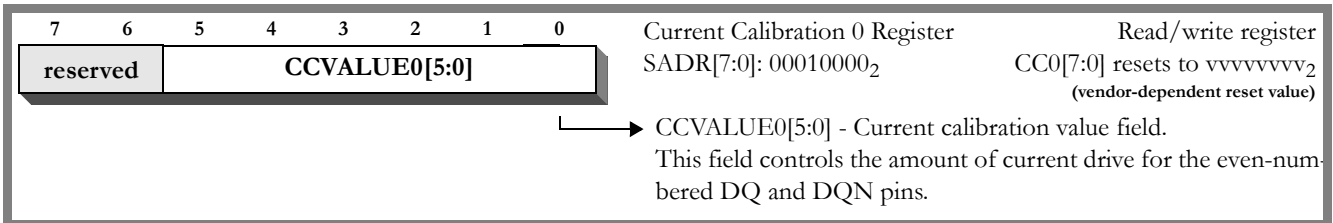
Figure 28 Current Calibration 0 (CC0) Register
