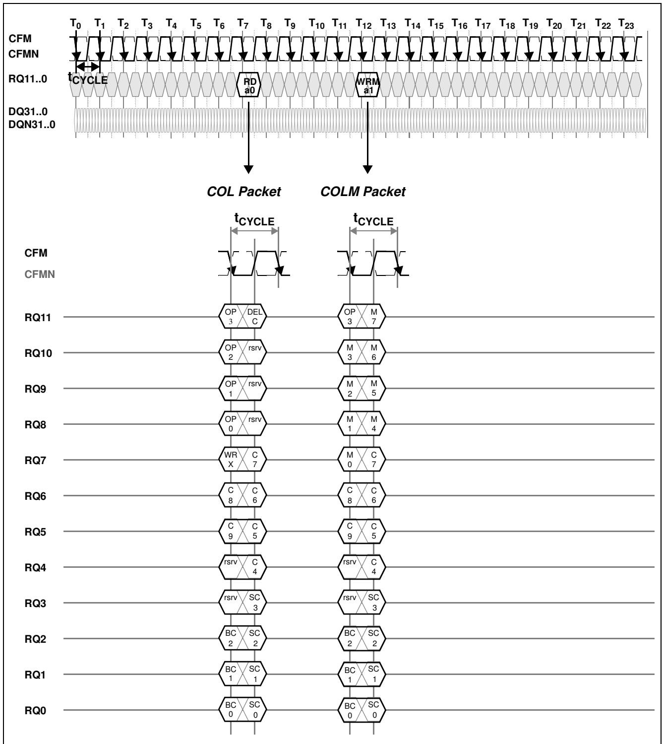
Figure 48 Alternate Request Packet Formats
