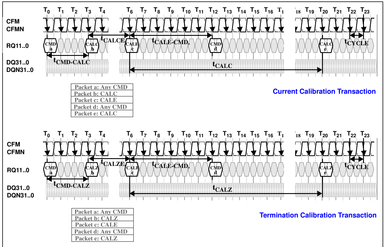
Figure 35 Calibration Transactions
