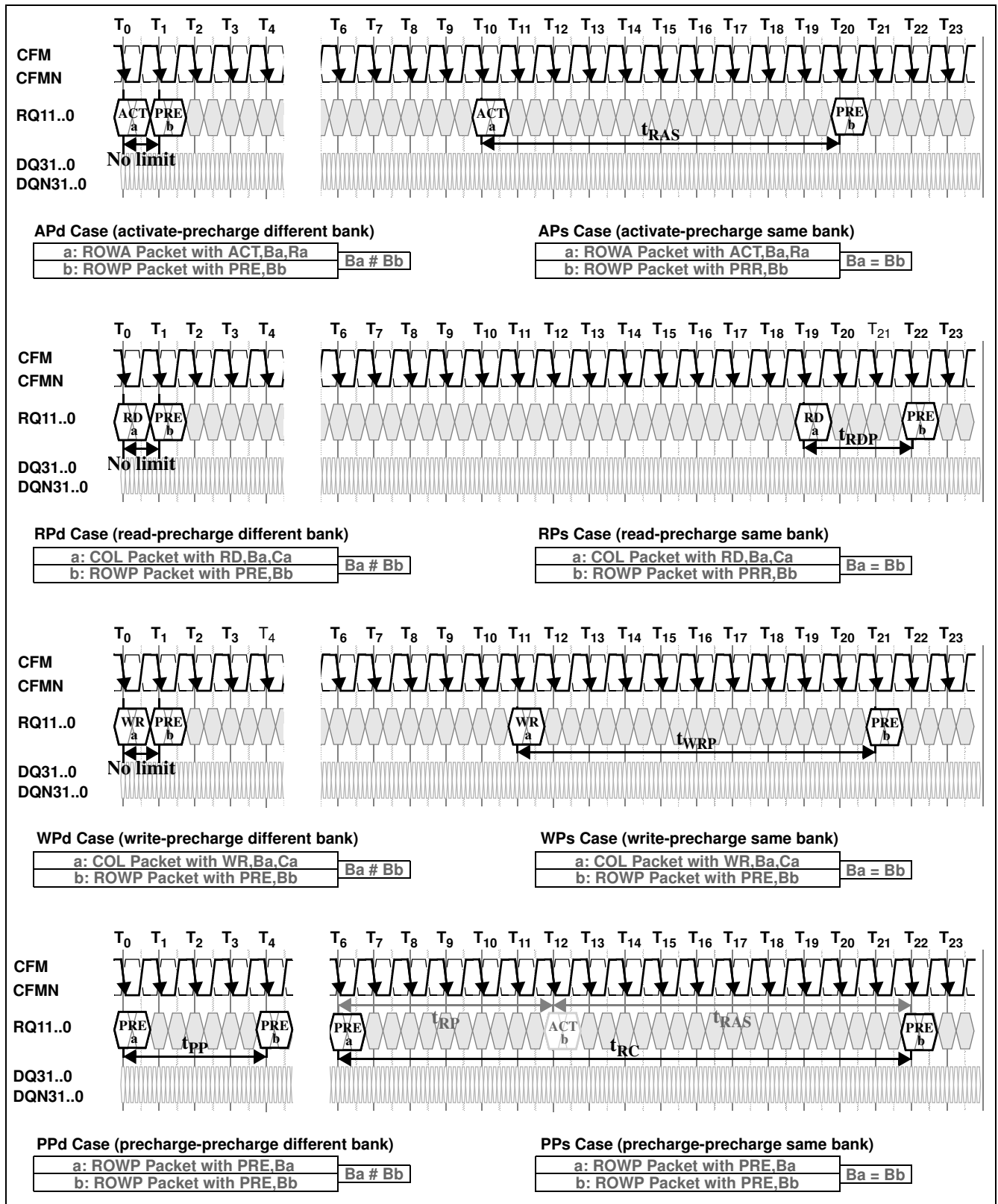
Figure 6 ACT-, RD-, WR-, PRE-to-PRE Packet Interactions
