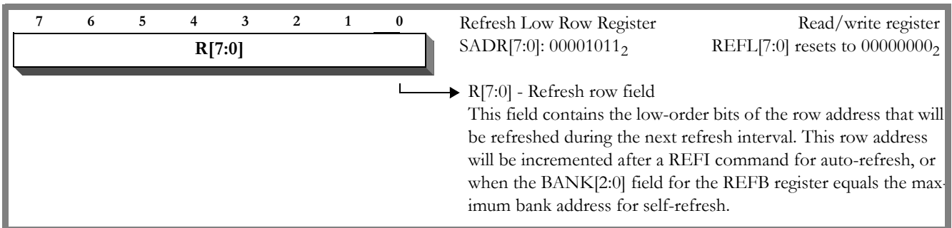
Figure 25 Refresh Low (REFL) Row Register
