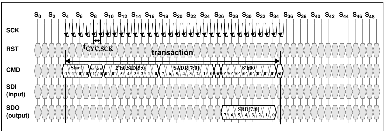
Figure 14 Serial Read Transaction — Selected DRAM
