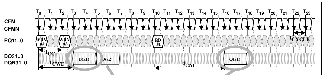
Figure 42 Write-Masked (WRM) Transaction Example
