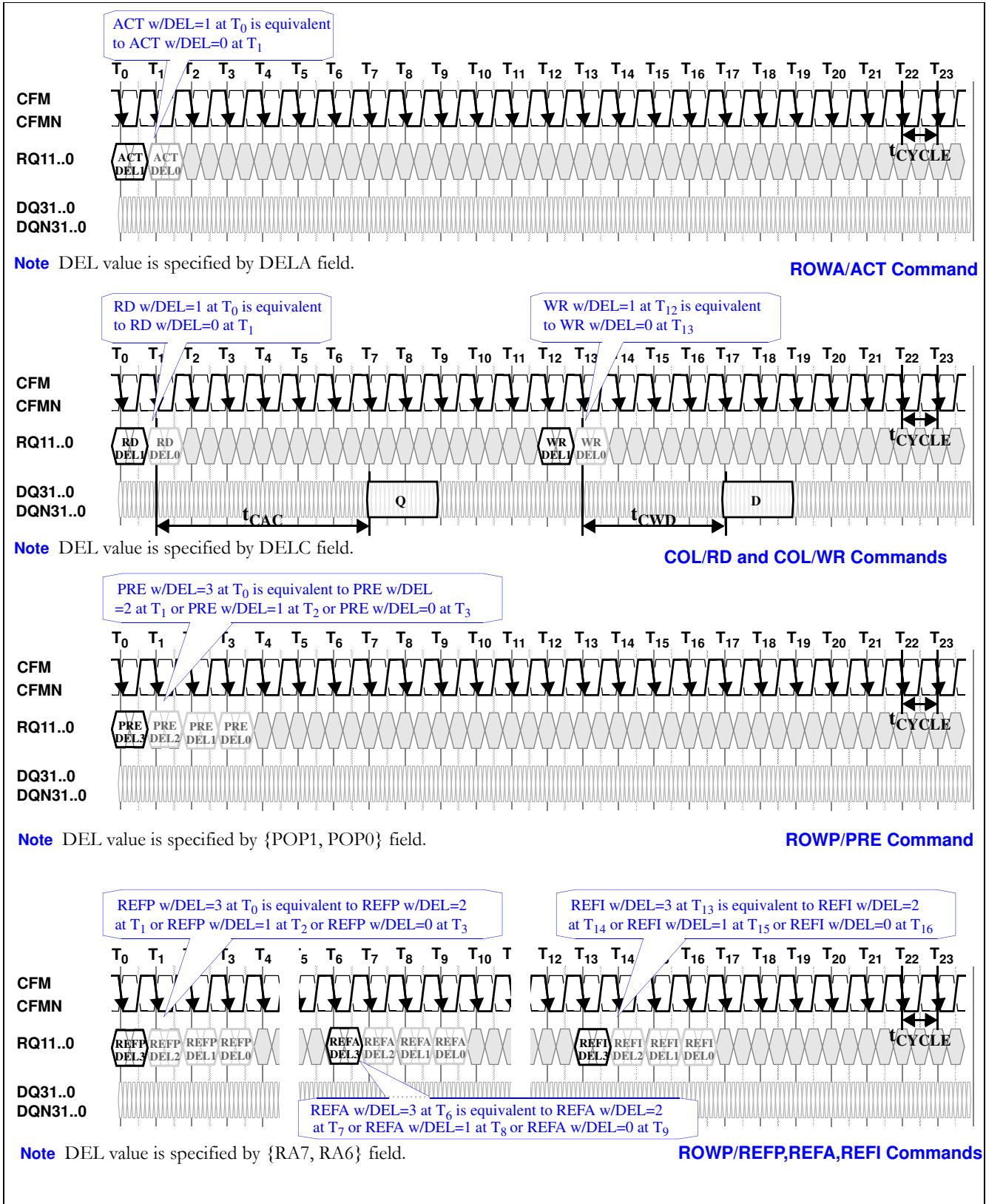
Figure 7 Request Scheduling Examples
