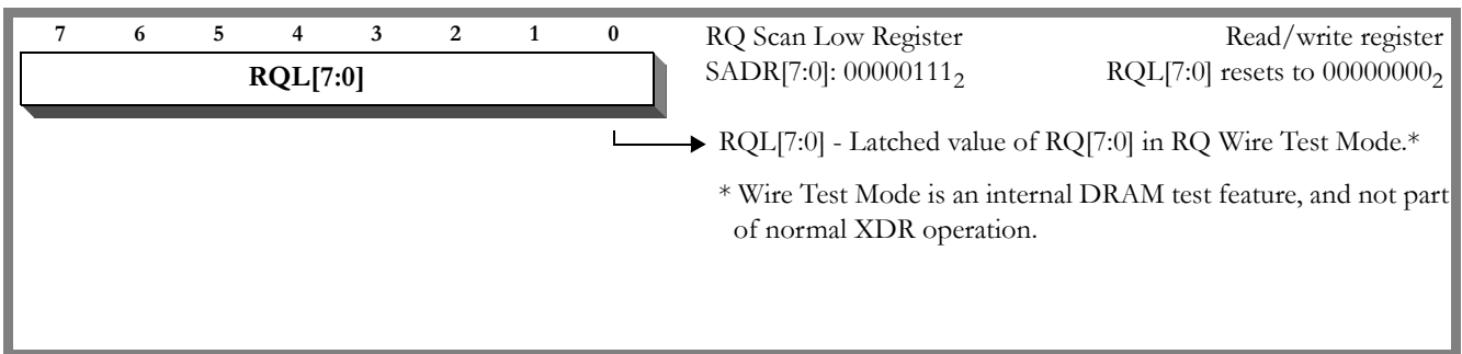
Figure 21 RQ Scan Low (RQL) Register
