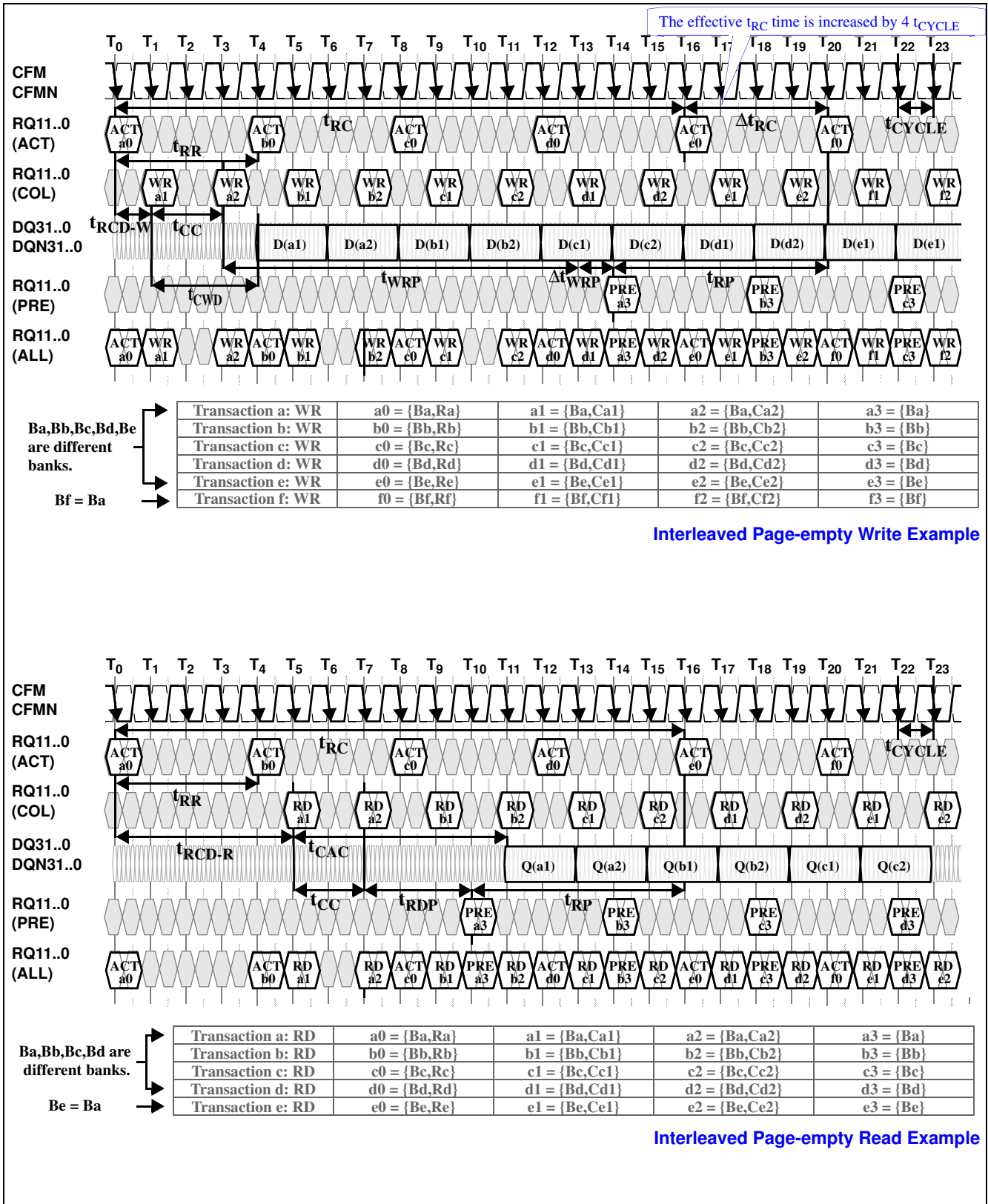
Figure 10 Interleaved Transactions
