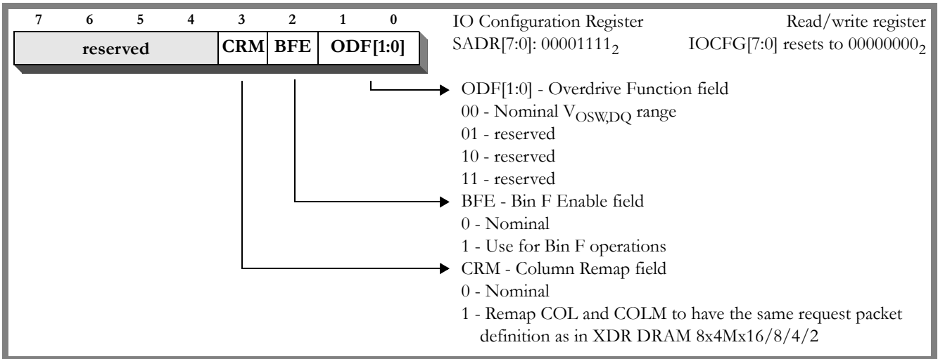
Figure 27 IO Configuration (IOCFG) Register
