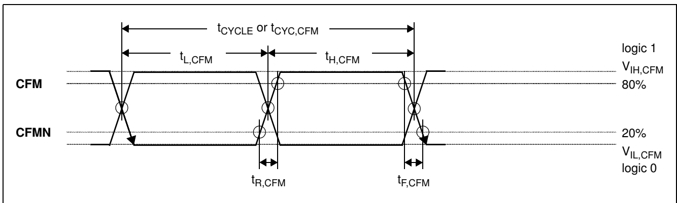
Figure 49 Clocking Waveforms
