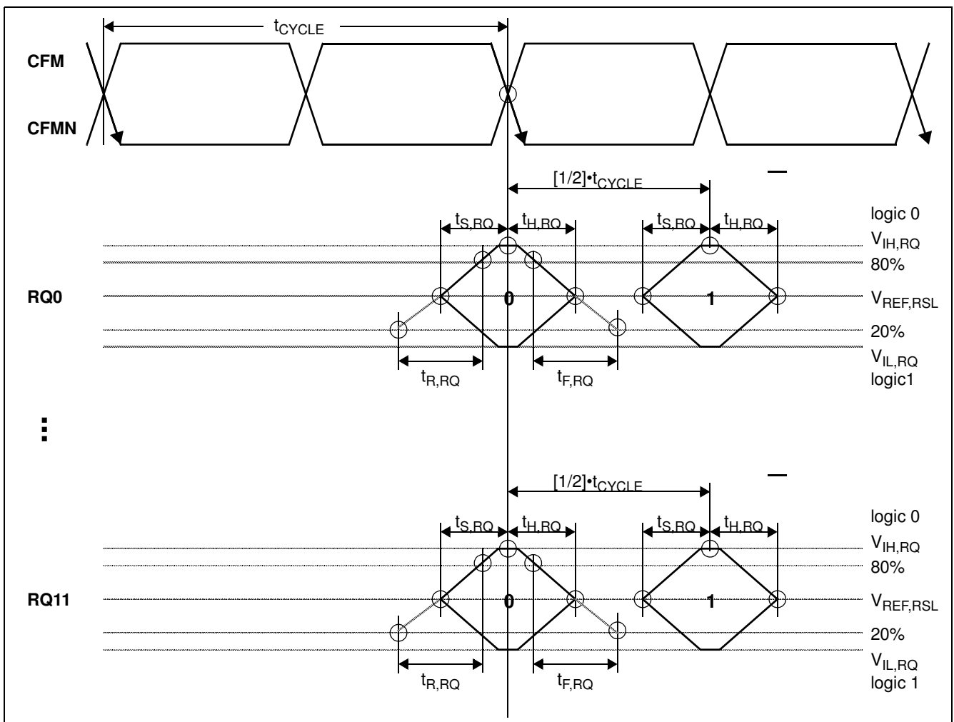
Figure 50 RSL RQ Receive Waveforms
