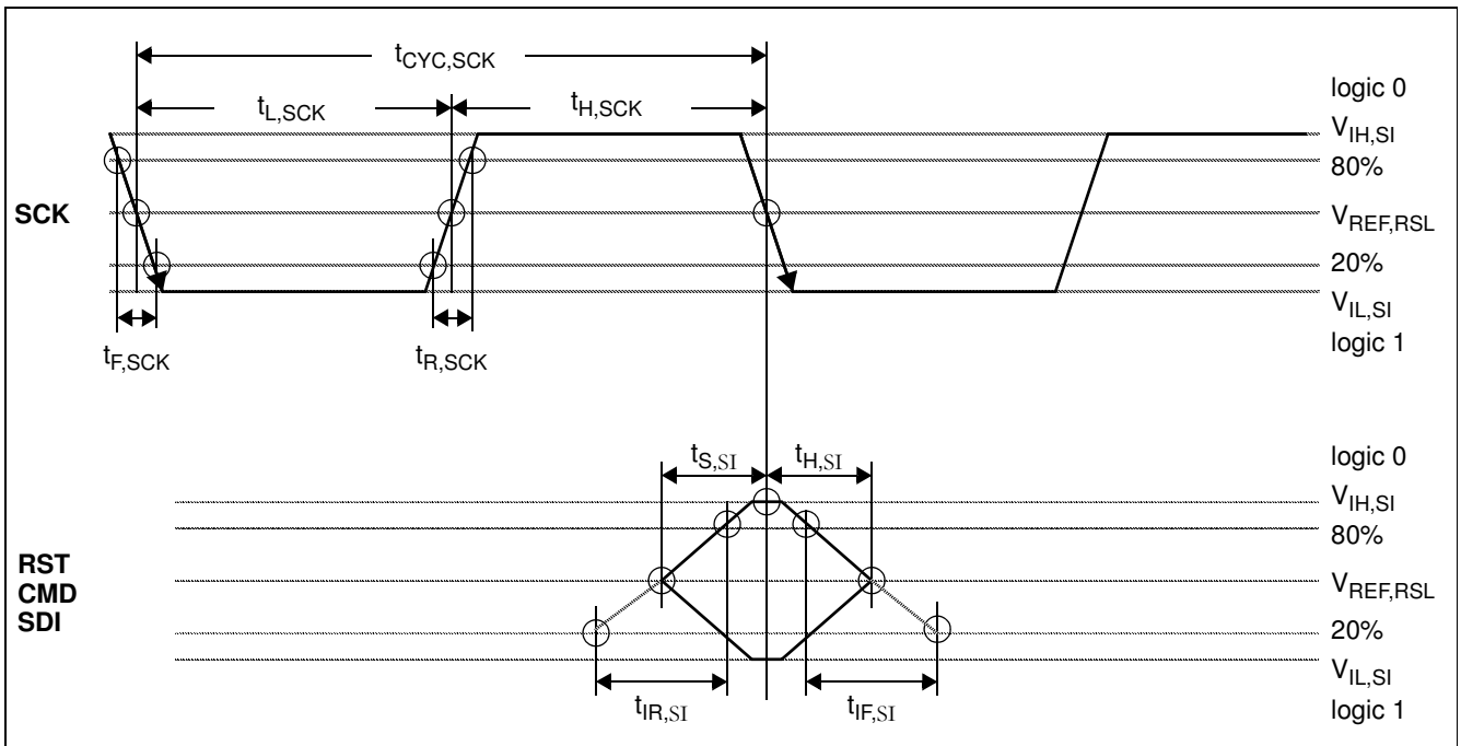
Figure 53 Serial Interface Receive Waveforms
