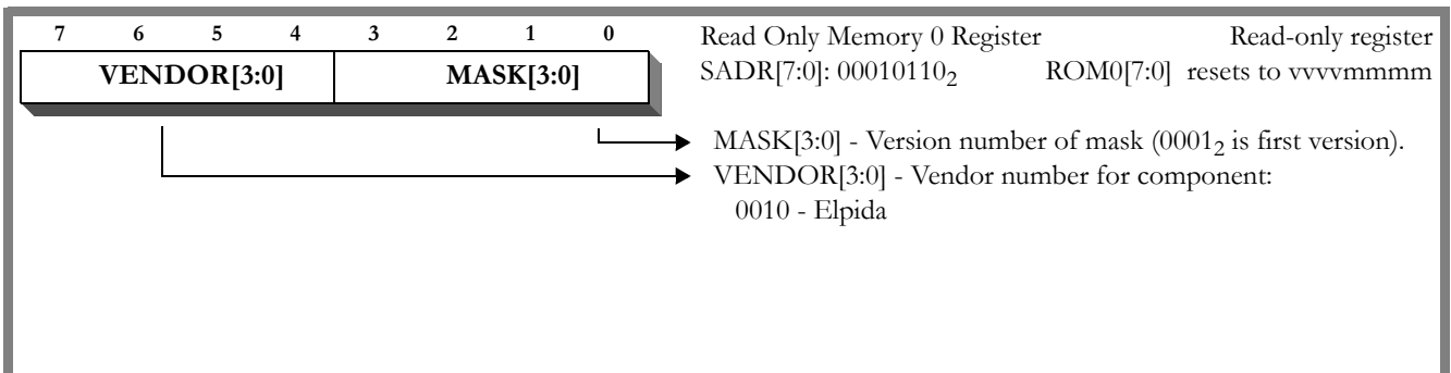
Figure 30 Read Only Memory 0 (ROM0) Register
