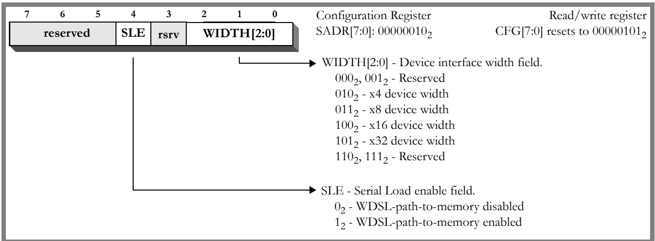
Figure 17 Configuration (CFG) Register
