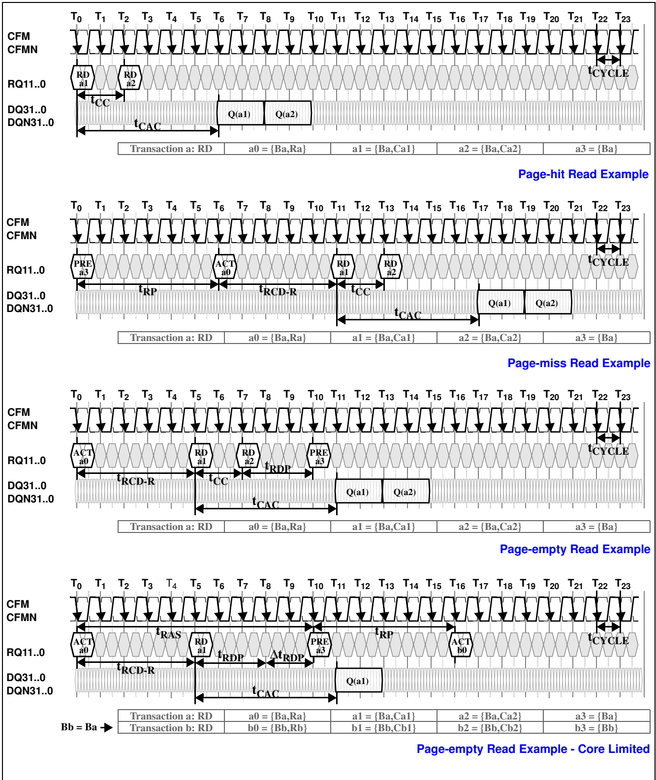
Figure 9 Read Transactions
