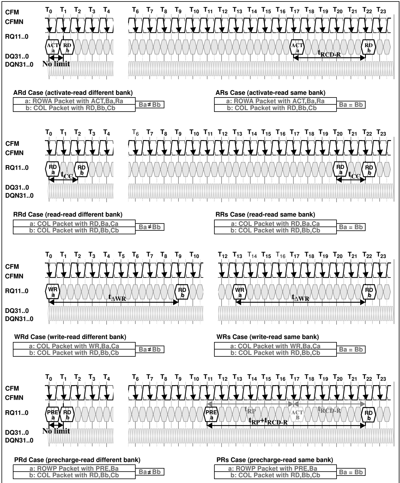
Figure 4 ACT-, RD-, WR-, PRE-to-RD Packet Interactions
