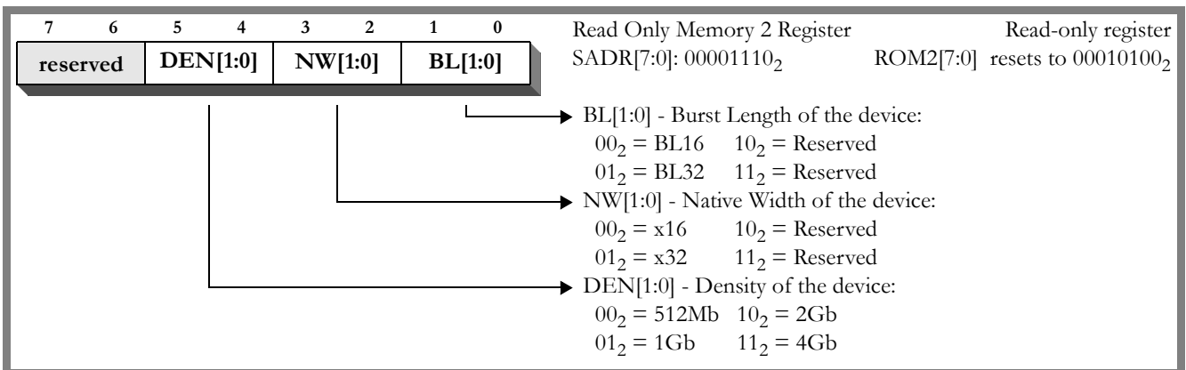
Figure 26 Read Only Memory 2 (ROM2) Register
