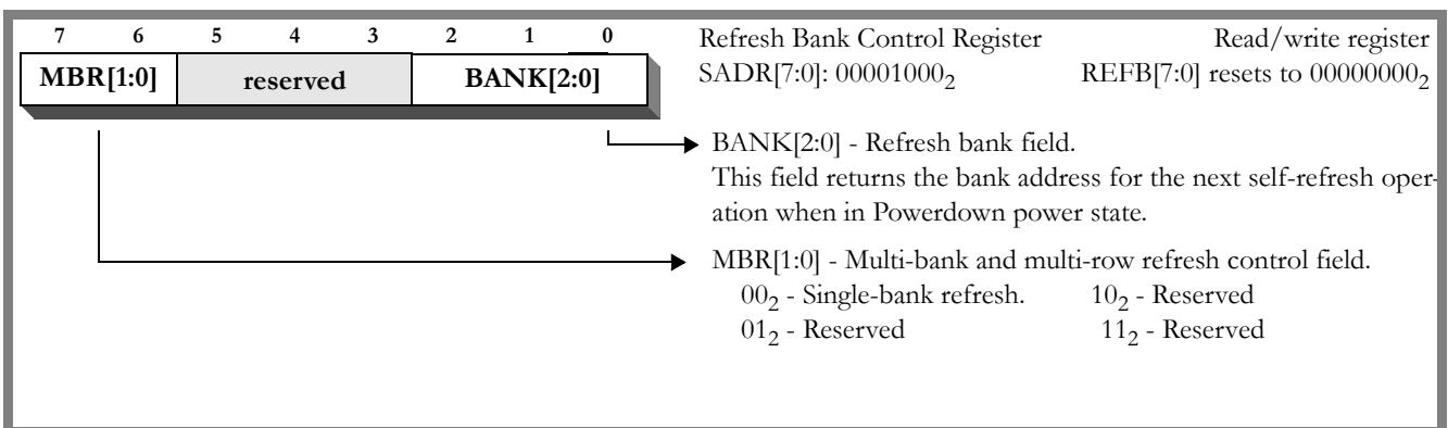
Figure 22 Refresh Bank (REFB) Control Register
