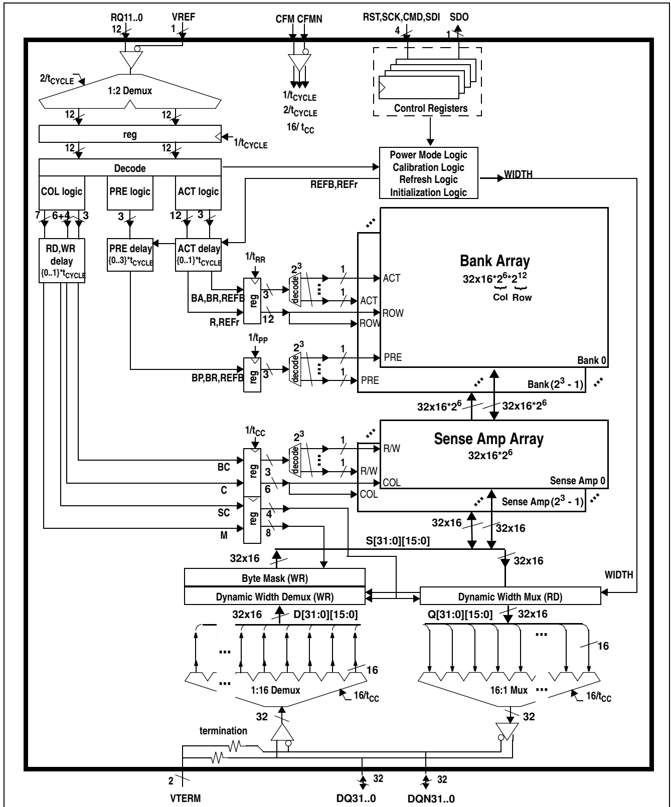
Figure 1 1Gb (8x4Mx32/16/8/4) XDR DRAM Block Diagram
