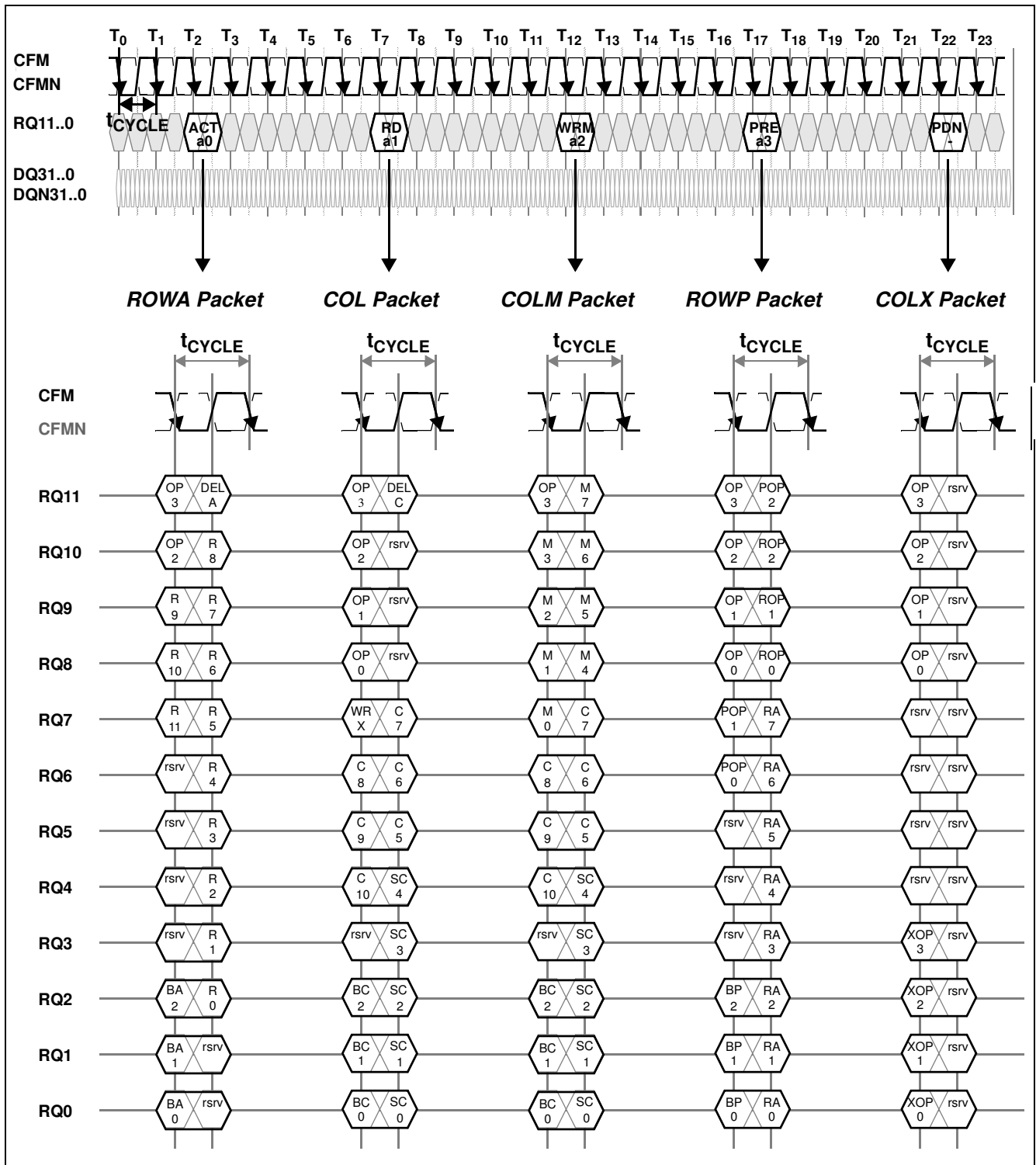
Figure 2 Request Packet Formats
