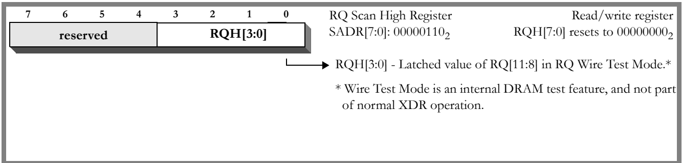
Figure 20 RQ Scan High (RQH) Register
