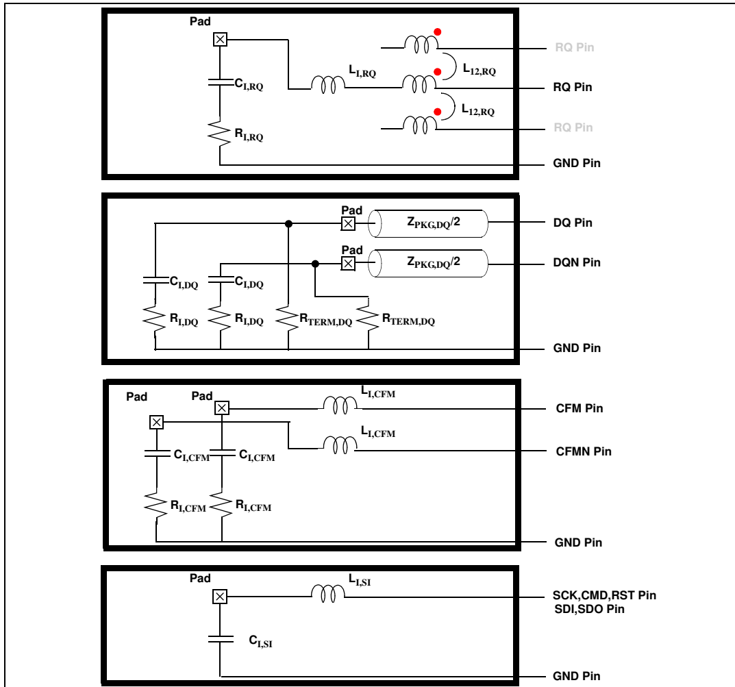
Figure 55 Equivalent Circuits for Package Parasitic
