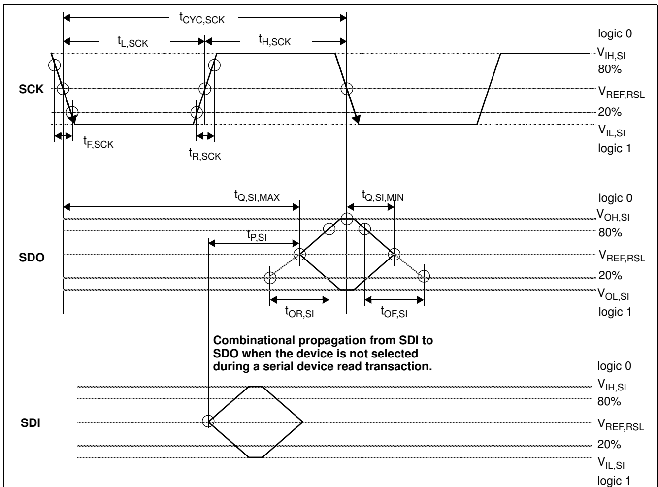
Figure 54 Serial Interface Transmit Waveforms
