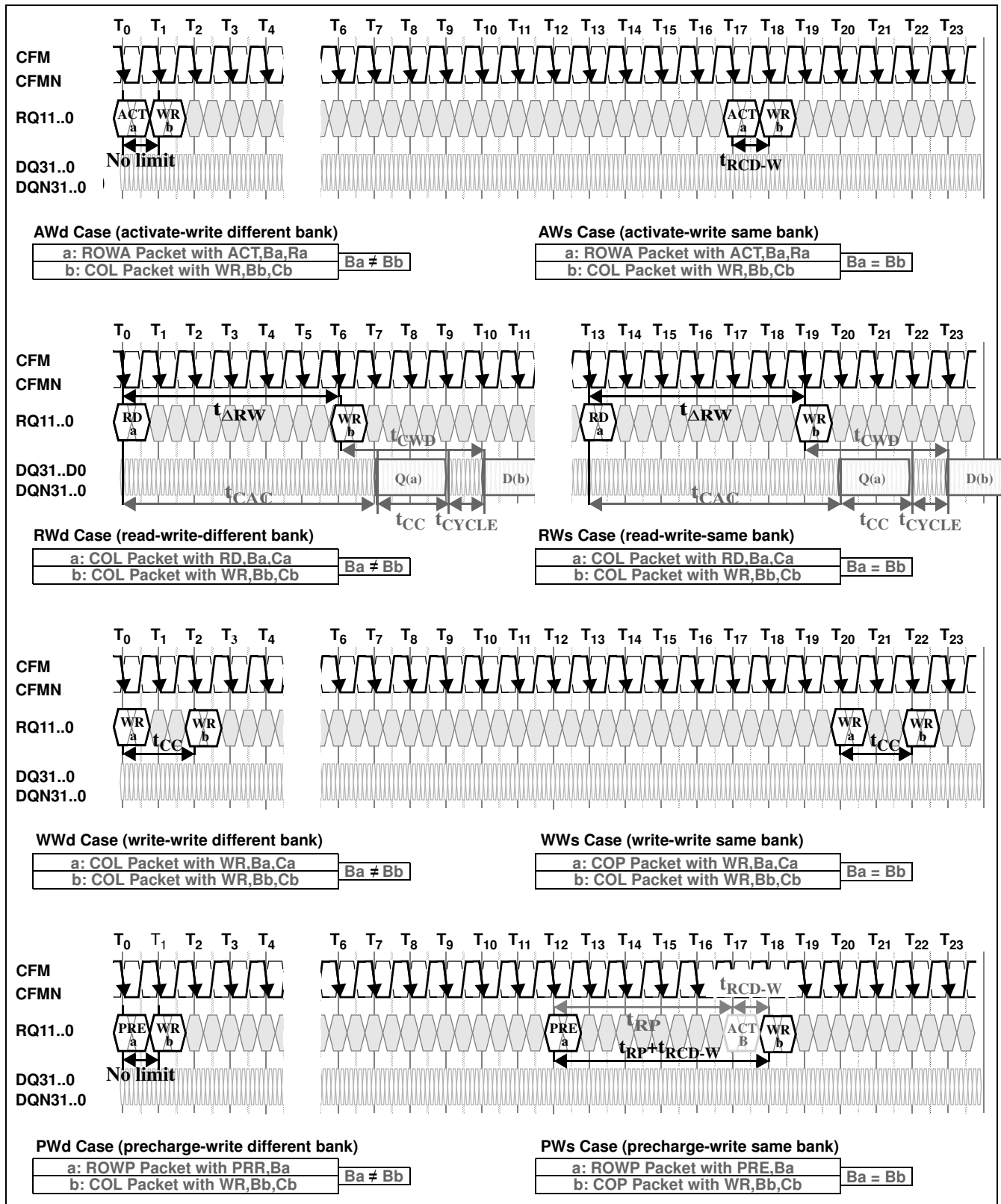
Figure 5 ACT-, RD-, WR-, PRE-to-WR Packet Interactions
