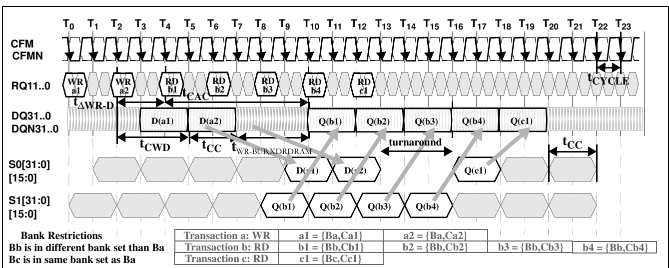
Figure 44 Write/Read Interaction — ERAW Feature
