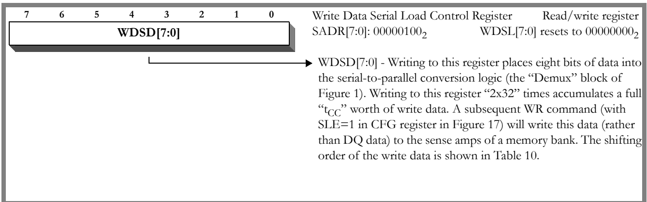
Figure 19 Write Data Serial Load (WDSL) Control Register
