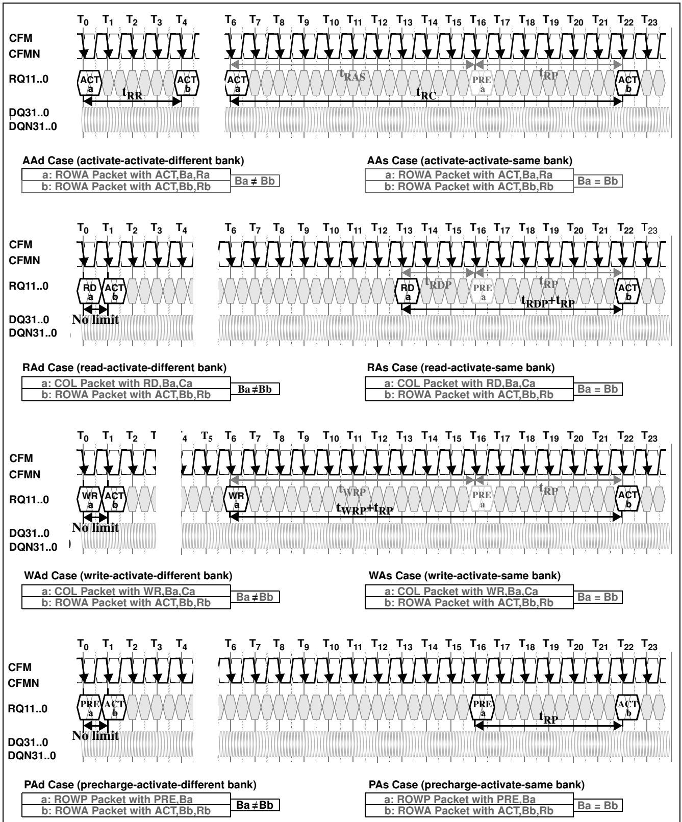
Figure 3 ACT-, RD-, WR-, PRE-to-ACT Packet Interactions
