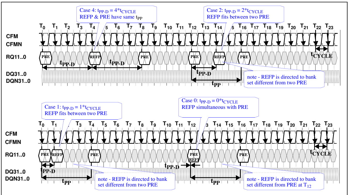
Figure 47 Simultaneous Precharge — t_{pp-D} Cases
