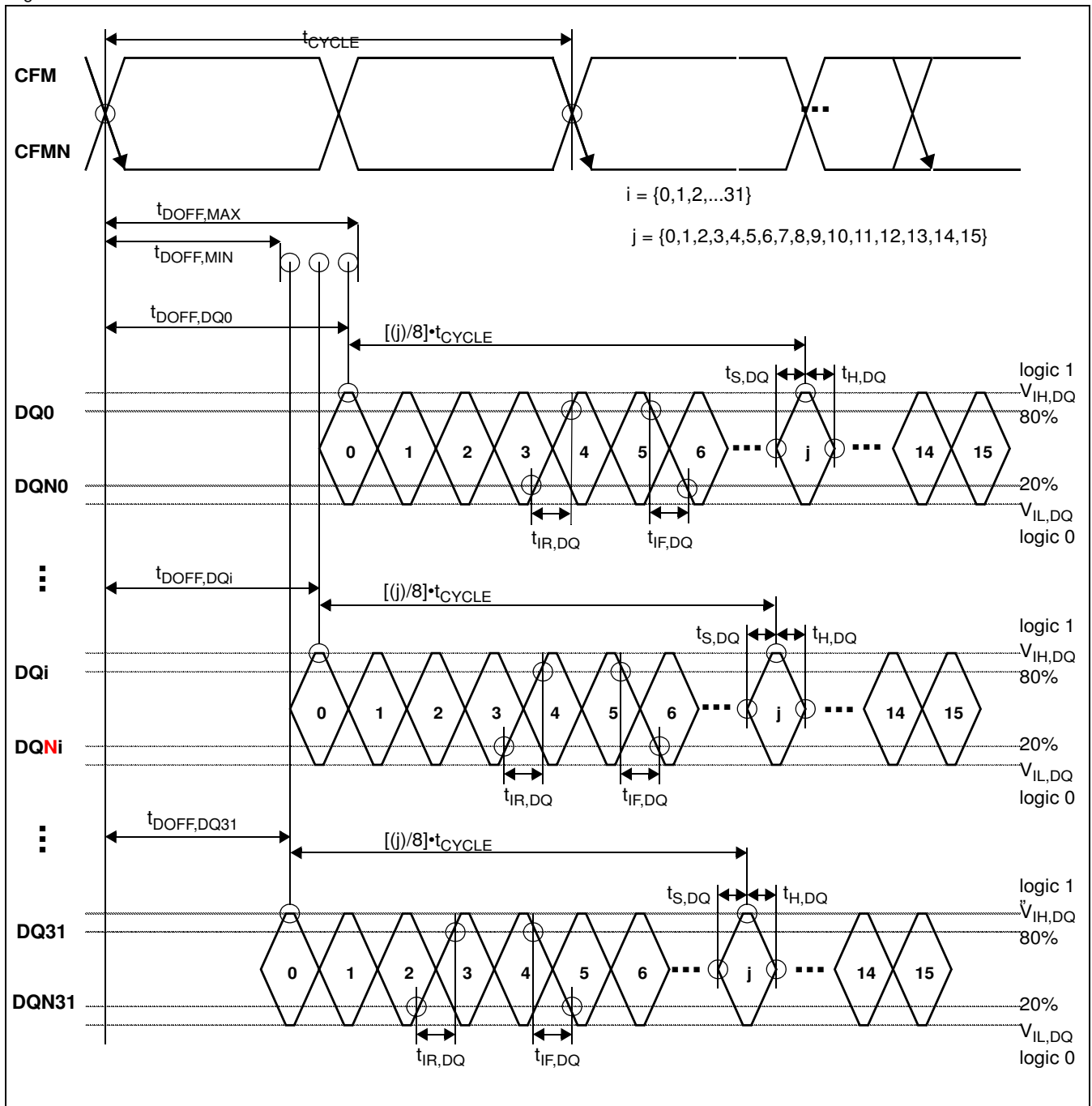
Figure 51 DRSL DQ Receive Waveforms
