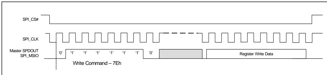
Figure 3.11 SPI Write Data Command - Bi-directional Mode
