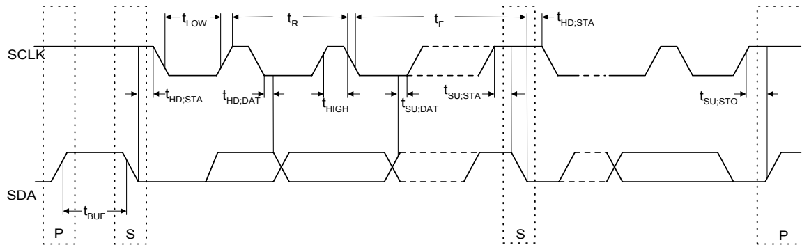
Figure 9.2 SMBus Timing
