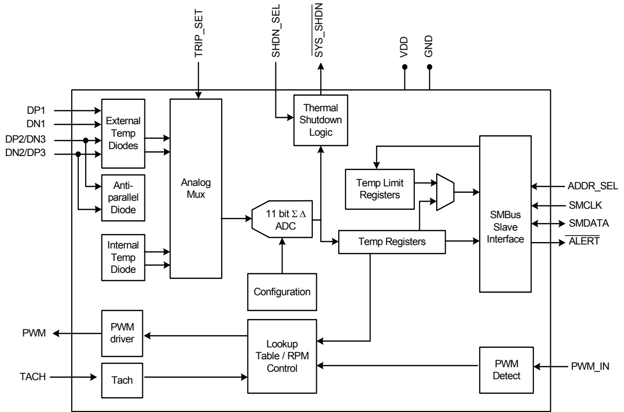
Figure 1 EMC2113 Block Diagram
