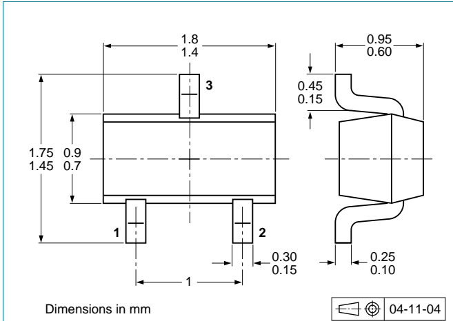
Fig 12. Package outline PDTA144EE (SOT416/SC-75)
