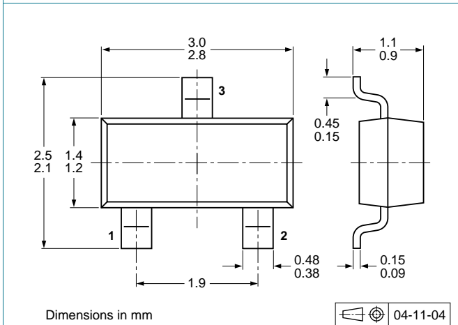
Fig 14. Package outline PDTA144ET (SOT23)
