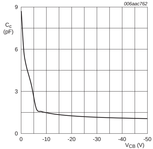
Fig 6. Collector capacitance as a function of collector-base voltage; typical values of built-in transistor
