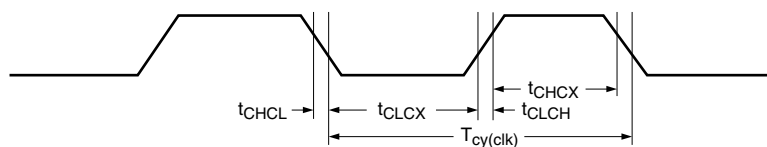
Fig 38. External clock timing (with an amplitude of at least V_{i(RMS)} = 200 mV)
