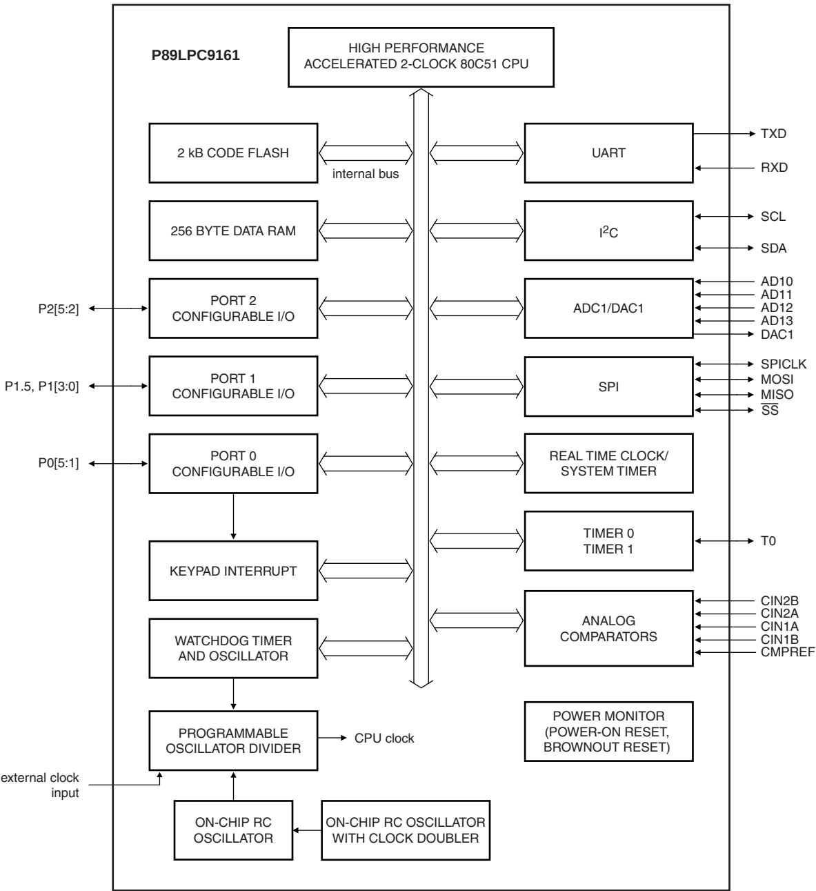
Fig 2. Block diagram (P89LPC9161)
