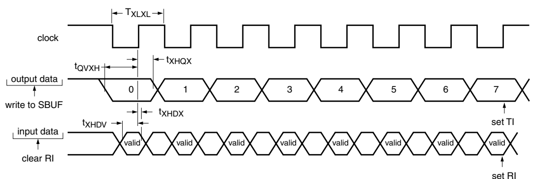
Fig 39. Shift register mode timing
