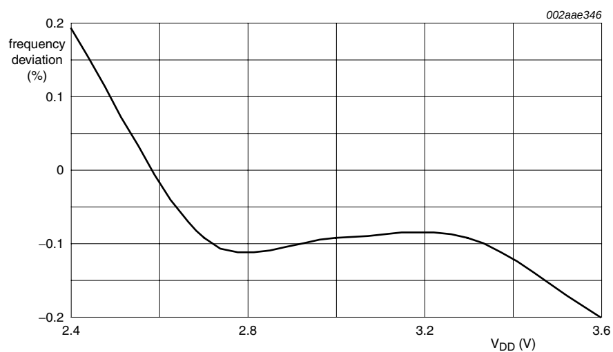
Fig 32. Average internal RC oscillator frequency versus V_{DD} at -40 °C
