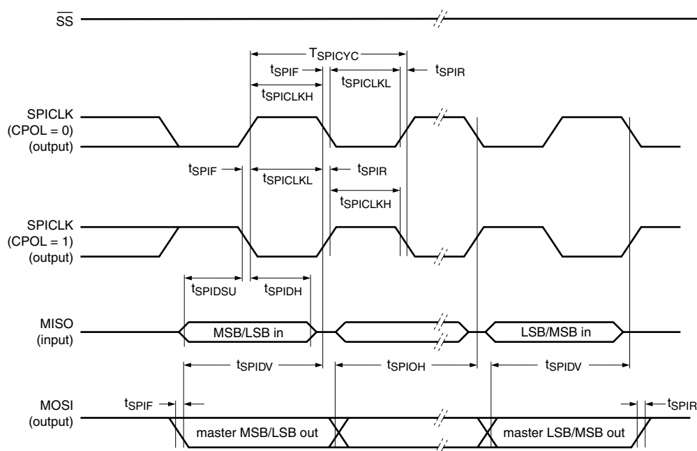
Fig 40. SPI master timing (CPHA = 0)
