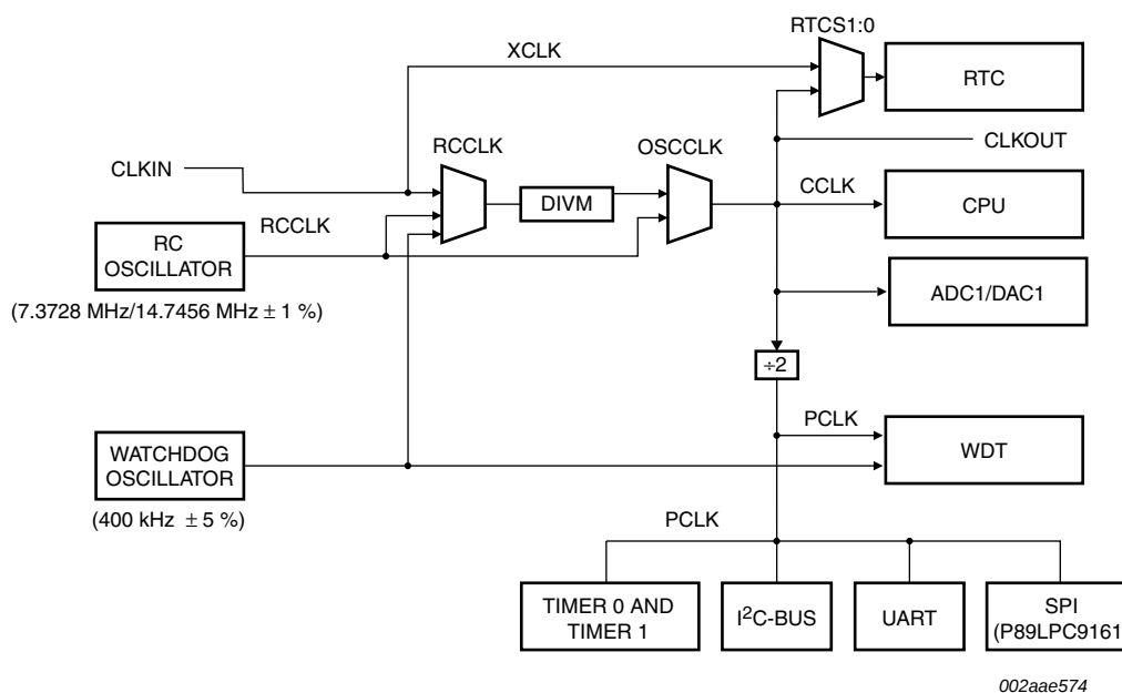
Fig 10. Block diagram of oscillator control
