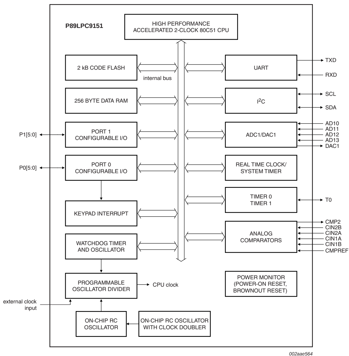
Fig 1. Block diagram (P89LPC9151)
