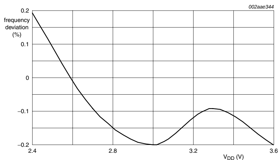
Fig 31. Average internal RC oscillator frequency versus V_{DD} at +25 °C
