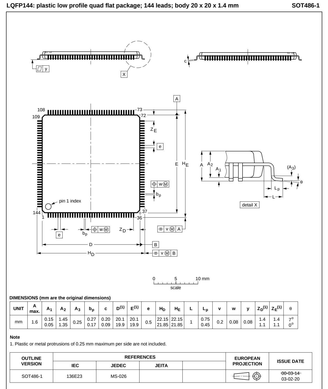
Fig 15. Package outline SOT486-1 (LQFP144)
