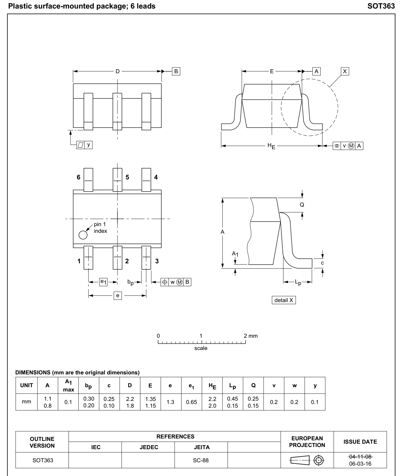
Fig 5. Package outline SOT363
