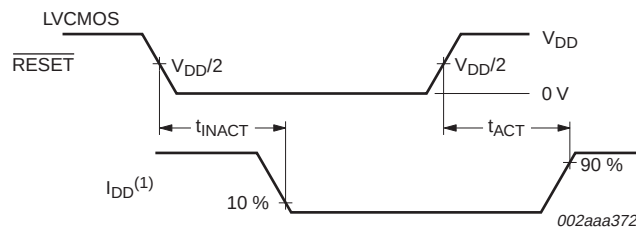
Fig 6. Inputs active and inactive times
