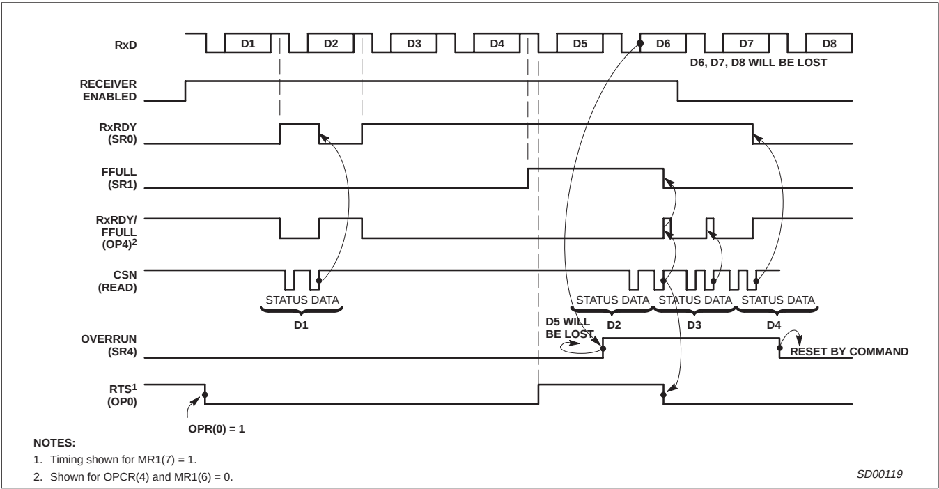
Figure 13. Receiver Timing
